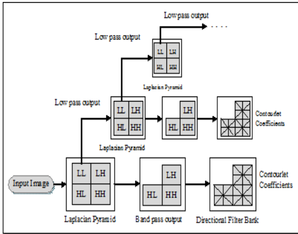
Figure (3). Decomposition of Contourlet transform.
