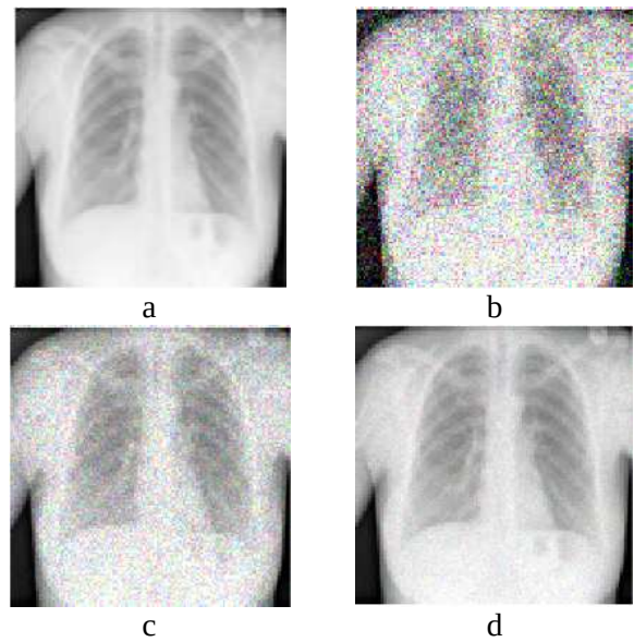
Figure (9). The visual results of x-ray image. (a) Original image (b) Noisy image by Gaussian noise (c) Noisy image by Speckle noise (d) Denoised image using CT.
