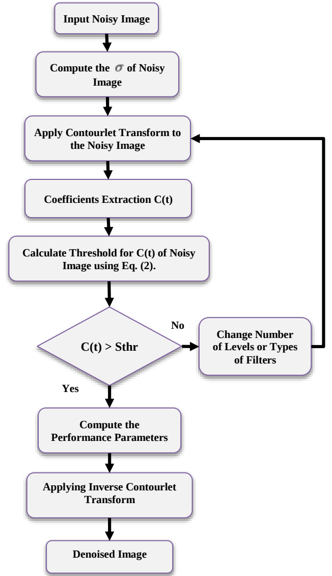
Figure (4). Block diagram of proposed algorithm.
