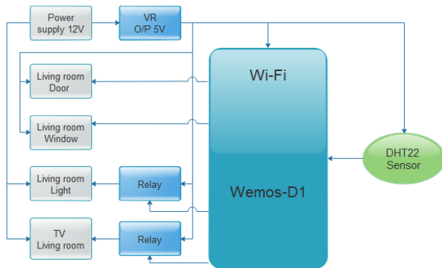
Fig. 13 The system third node schematic diagram.
