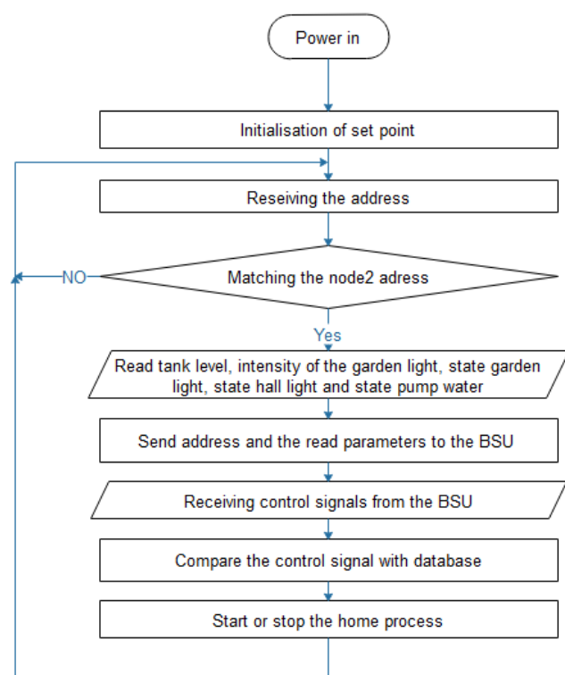
Fig. 26 second SU flowchart.
