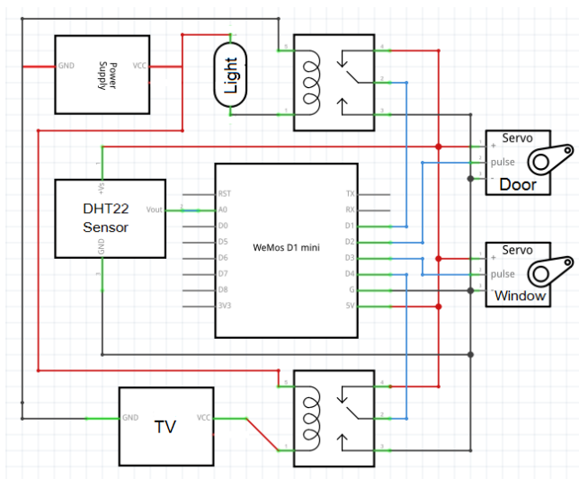
Fig.15. Interfacing schematic living room diagram.
