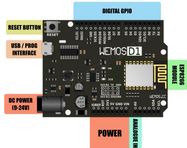
Fig. 6 Wemos-D1 Board.
