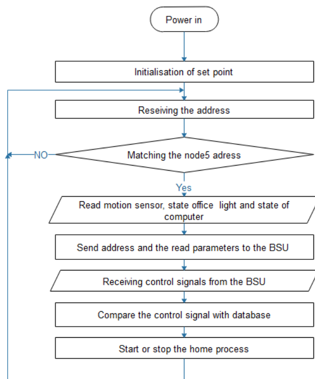
Fig. 29 fifth SU flowchart.
