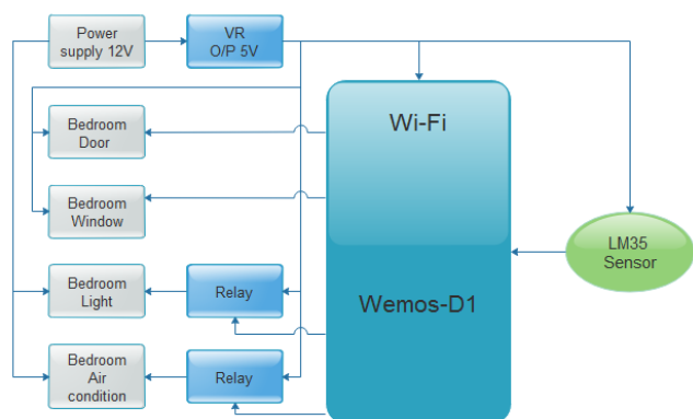
Fig. 7 The system first node schematic diagram.
