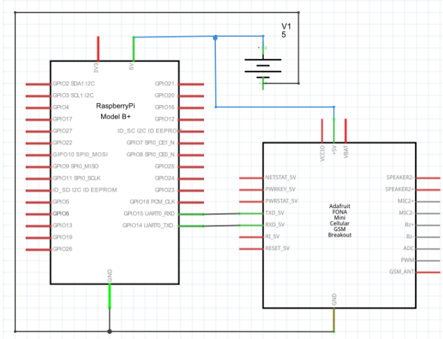
Fig. 5 Interfacing GSM with Raspberry pi board.
