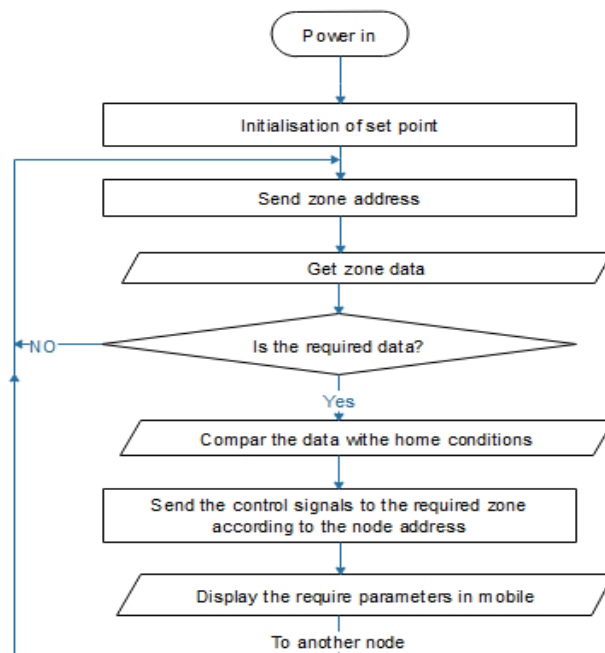
Fig. 24 BSU flowchart.
