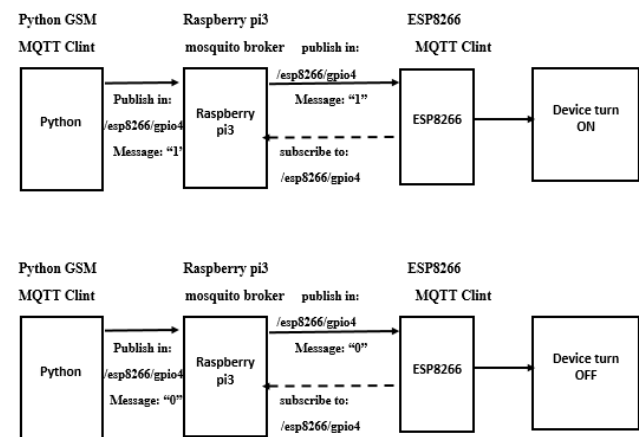
Fig.1. show overview of the system
