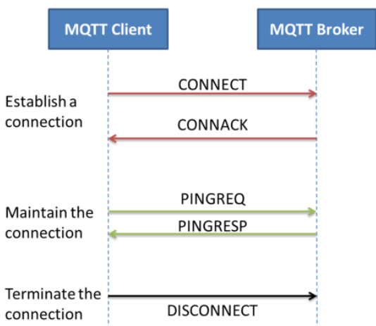
Fig. 1. Establishing, maintaining and terminating MQTT connection
