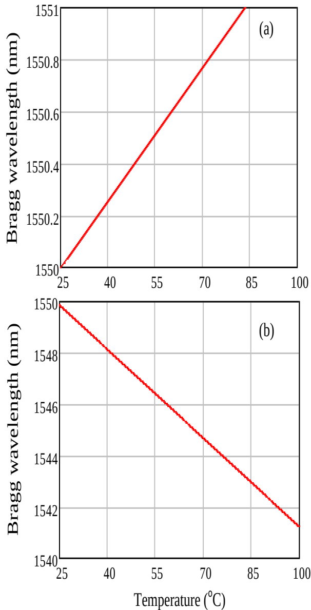
Figure 1 Temperature effect on Bragg wavelength of (a) Silica Optical Fiber (SOF) and (b) Polymer Optical Fiber (POF)
