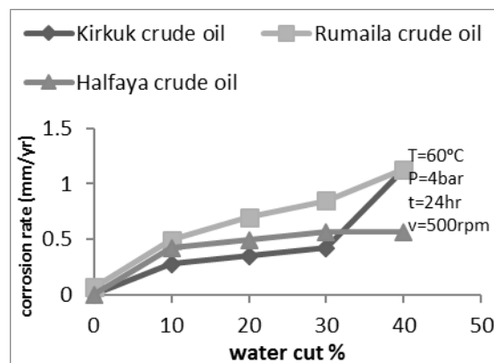
Fig. 7. Comparison of the corrosion rates of carbon steel in three Iraqi crude oil/produced water, 3
