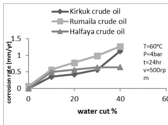
Fig. 6. Comparison of the corrosion rates of carbon steel in three Iraqi crude oil/produced water, 2% NaCl
