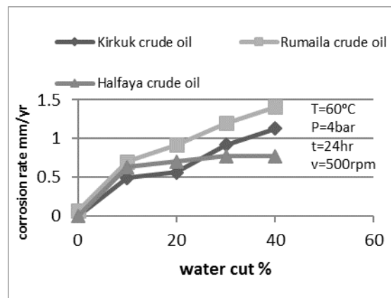
Fig. 5. Comparison of the corrosion rates of carbon steel in three Iraqi crude oil/produced water, 1% NaCl.
