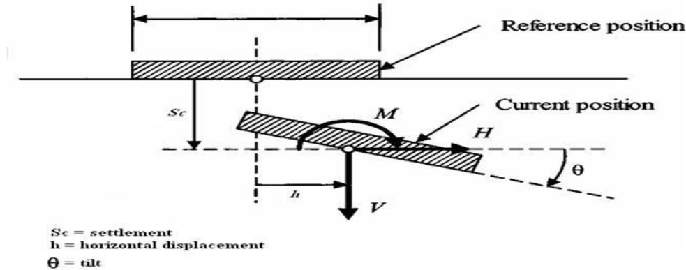
Fig. 1. Shallow Foundation Subjecte to eccentric-inclined load (after Butterfield et al. 1997)
