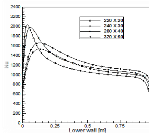
Fig.2. Grid independence test results
