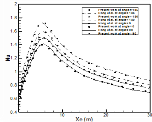
Fig.4. Comparison of Nusselt Number with the results of Hong et al. [18] ( S=4.8 mm, and ER=2 ) for Re=100 , and q_w=200 W/m^2 at different inclination angles
