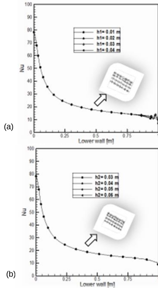
Fig. 14. Nusselt number for different steps heights of two steps (a) first step h_1 , and (b) second step h_2 of \text{SiO}_2 nanofluid at \text{Re} = 1000
