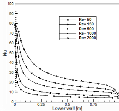
Fig. 10. Local Nusselt number along the heated bottom wall for different Reynolds numbers of \text{SiO}_2 nanofluid with laminar flow at \phi = 4\% and d_p = 20 nm
