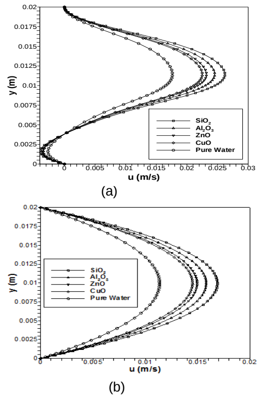
Fig. 7. Velocity distributions of different nanofluids with \phi=4\% for Re=1000 , d_p=20 nm and at (a) X/H = 9 , (b) X/H = \text{Exit}
