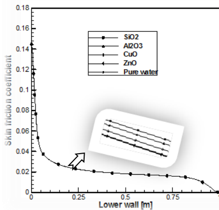
Fig. 6. Skin friction coefficient for different nanofluids along the heated bottom wall Re=1000 with d_p=20 nm and \phi=4\%
