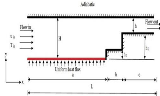
Fig.1. Schematic diagram for 2D FFS in a channel flow
