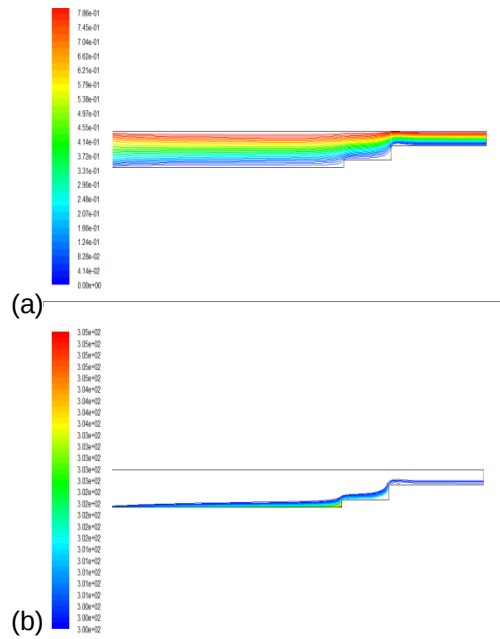
Fig. 13. Streamlines (a) and isotherms (b) for \text{Re}=2000 of \text{SiO}_2 nanofluids flow with \phi = 4\% , d_p = 20 nm
