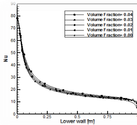
Fig.9. Local Nusselt number for different volume fractions along the heated bottom wall of \text{SiO}_2 nanofluids flow \text{Re} = 1000 at d_p = 20 nm
