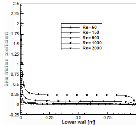
Fig. 11. Skin friction coefficient along the heated wall for different bottom wall for different Reynolds numbers of \text{SiO}_2 nanofluid with laminar flow at \phi = 4\% and d_p = 20 nm
