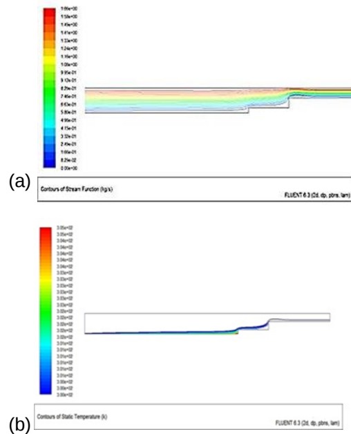
Fig. 8. (a) Streamlines and (b) isotherms for SiO_2 nanofluids flow with \phi = 4\% for Re = 1000 , d_p = 20 nm
