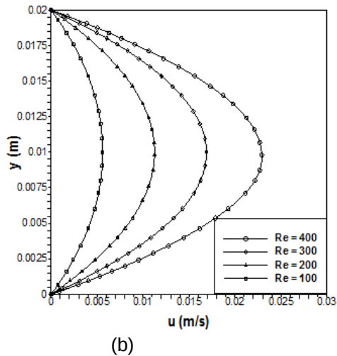
Fig. 12. Velocity distribution of \text{SiO}_2 nanofluid for different Reynolds number with \phi = 4\% and d_p = 20 nm at (a) X/H = 9 , (b) X/H = \text{Exit}
