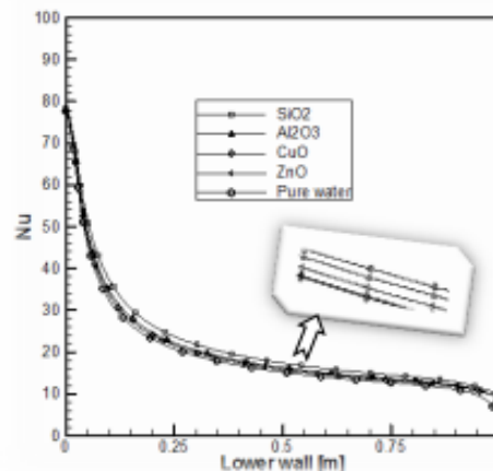
Fig. 5. Local Nusselt number for different nanofluids along the heated bottom wall Re=1000 with d_p=20 nm and \phi = 4\% .
