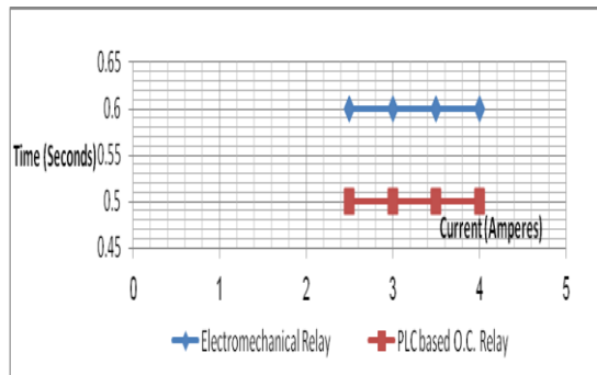
Fig. 11-a. Characteristics of Instantaneous Over Current protection (ITOC)
