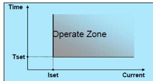
Fig. 5. Operating zone of definite time protection
