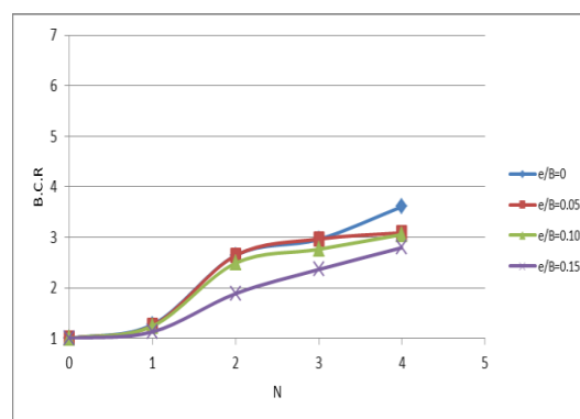
Fig. 10. Bearing capacity ratio versus number of reinforcement layer for (e/B = 0, 0.05, 0.10 and 0.15) and (RD=80%)
