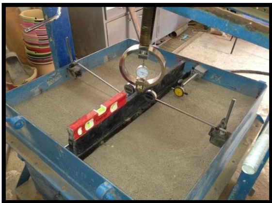
Fig. 4. A steel plate model which transfer distributed line load on the strip footing
