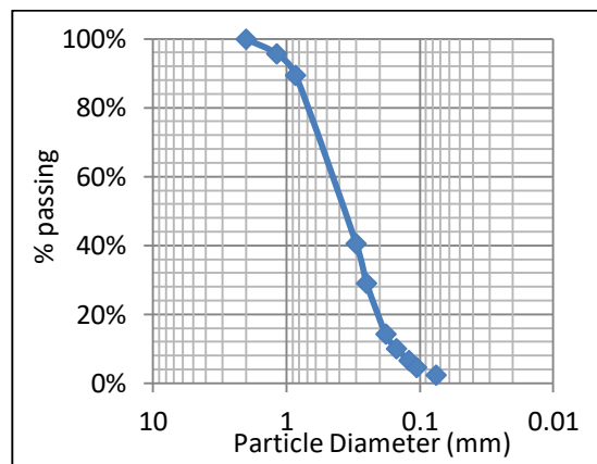
Fig. 5. Particle Size Distribution of the sand
