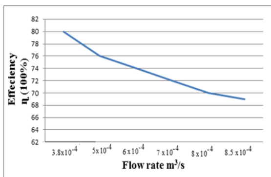
Fig. 3. Relationship between efficiency and flow rate of fluid.
