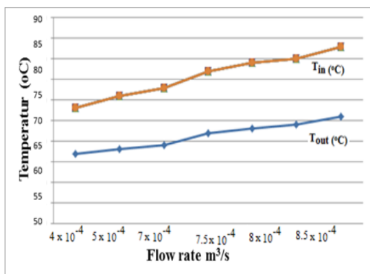
Fig. 4. Effect of flow rate on the Input and output primary temperature of heat exchanger
