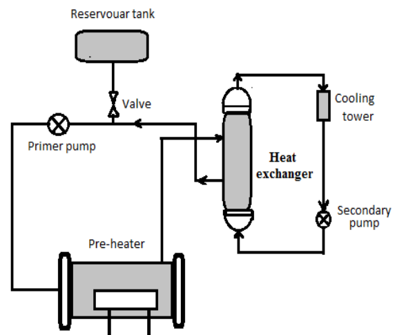
Fig. 1 : Block Diagram of BETA loop circuit.
