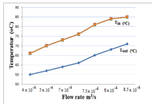
Fig. 5. The variations of input and output of the secondary temperature and flow rate of fluid
