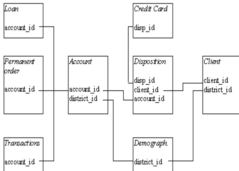
Figure(1) Relational Structure Schema Of Experimented data
