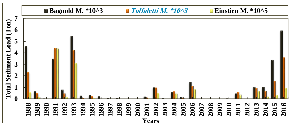
Fig. 6. Annual sediment load of Crnold valley.
