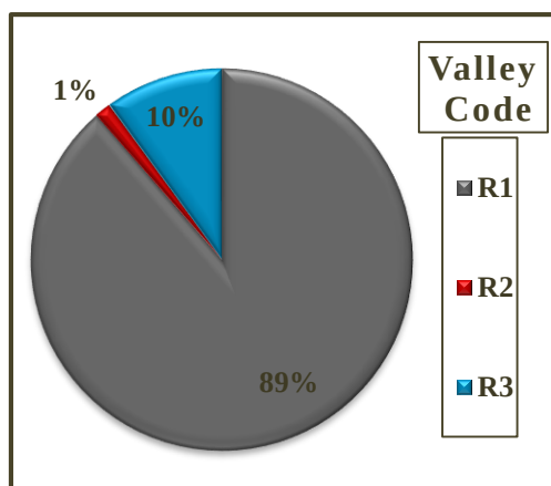
Fig. 8. The percentage of sediment load delivered to the right side of the lake using the average of the three methods used in this study.
