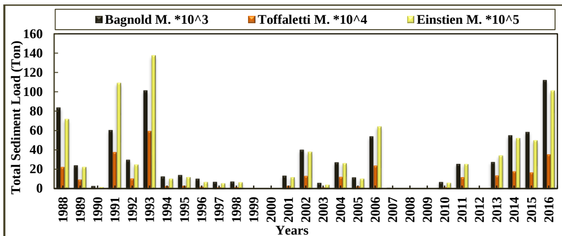
Fig. 5. Annual sediment load of Sweedy valley.
