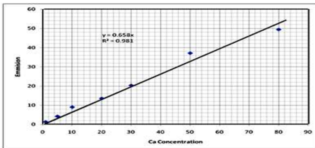
Fig (4): Calibration curve for Calcium determination by flame emission photometry
