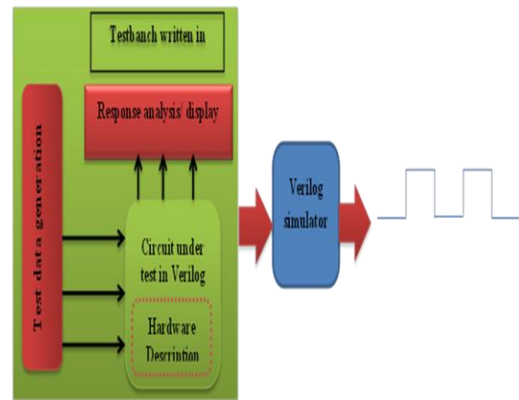
Fig. 5. Process of simulations in Verilog.
