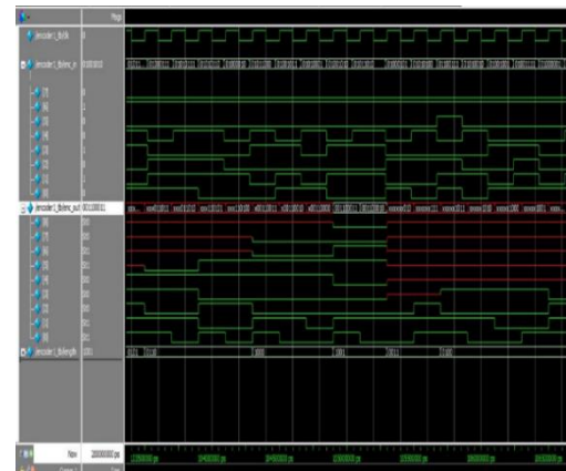
Fig. 8. Decoder Simulation.
