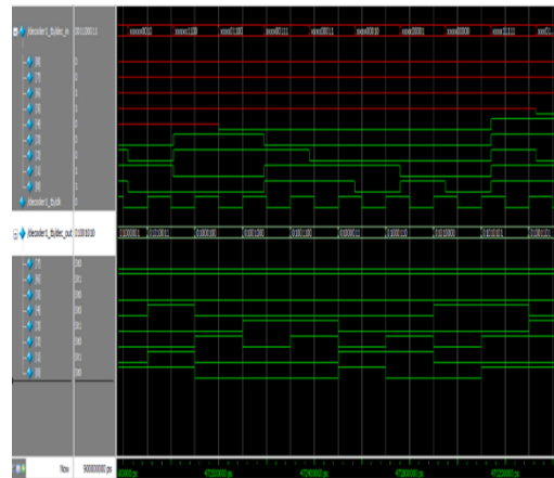
Fig. 7. Encoder simulation.
