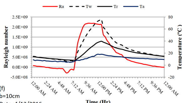
Fig. 6. Variation of Ra number and temperature change inside a test rig according to the ambient temperature for different width air gap channel during 24 hrs.
