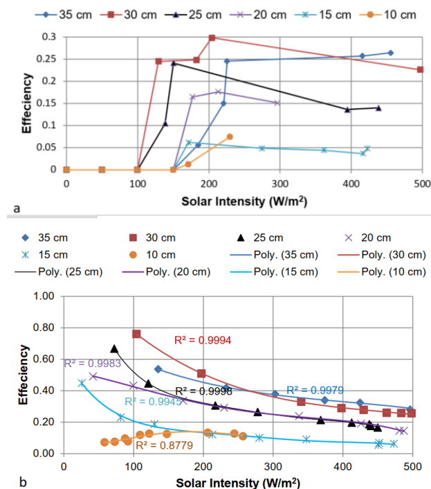
Fig. 7. The efficiency of the Trombe wall vs. solar intensity for different widths of the air gap. (a) before afternoon, and (b) after afternoon.
