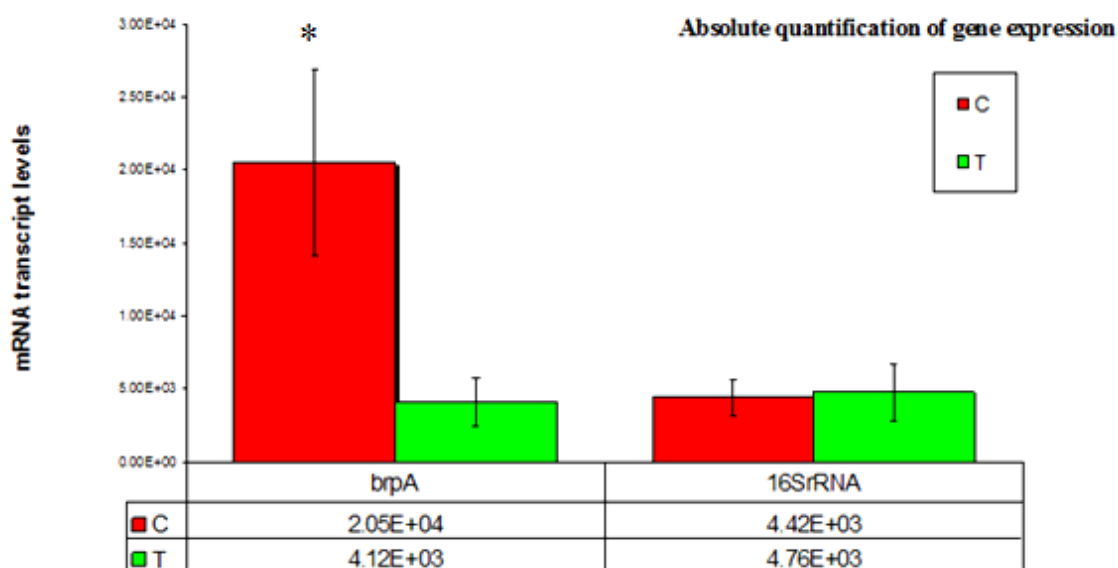
Figure (6): Absolute quantification gene expression of target gene ( brpA ) and house keeping gene ( 16S rRNA ) in S. mutans isolates.
