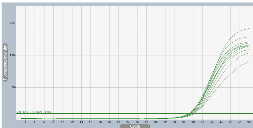
Figure (3): Real-Time PCR amplification plot of housekeeping gene (16S rRNA) in treatment and control S. mutans isolates.
