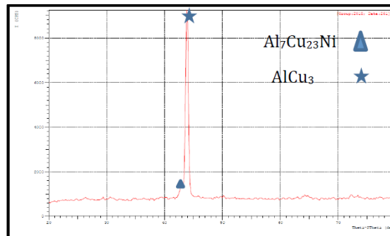
Figure 2: The results of (XRD) for the S1 shape memory alloy.
