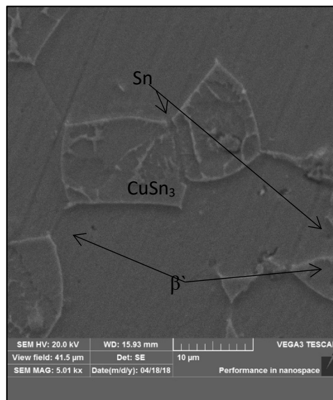
Figure 8: The (S3) alloy microstructure.
