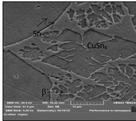
Figure 7: The (S2) alloy microstructure.
