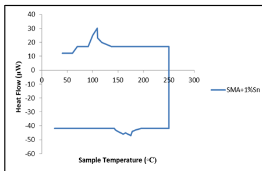
Figure 12: Thermogram of (S2) SMA.
