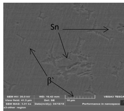
Figure 6: The (S1) alloy microstructure
