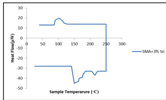
Figure 13: Thermogram of (S3) SMA.
