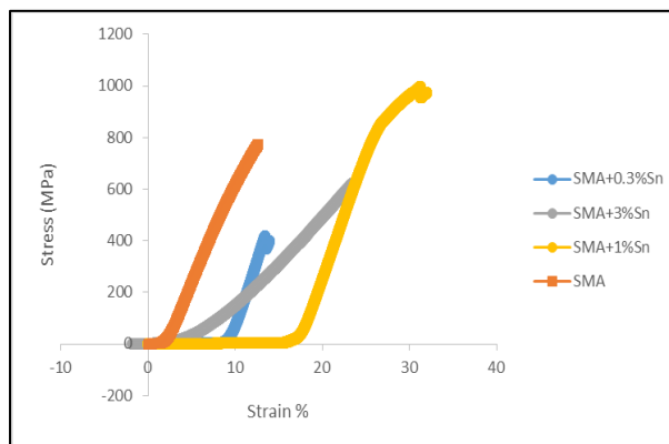
Figure 14: Stress – Strain Diagram.
