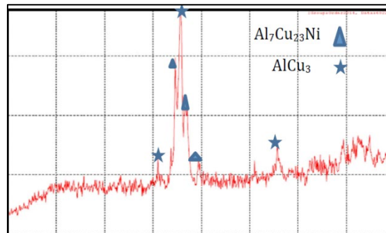
Figure 1: The results of (XRD) for the base shape memory alloy.
