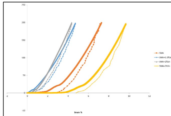
Figure 15: Thermo-Mechanical Stress –Strain Diagram.
