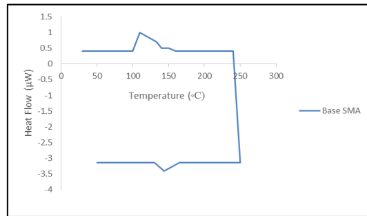
Figure 10: Thermogram of Base SMA.
