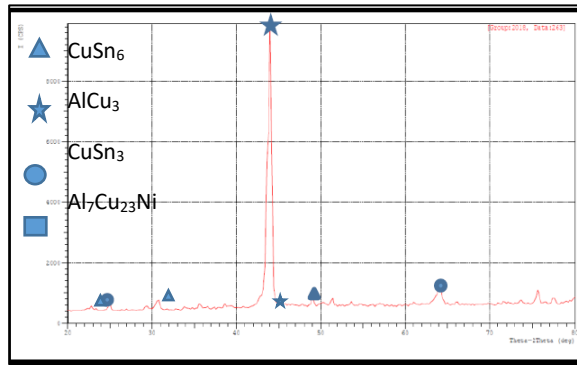
Figure 4: The results of (XRD) for the S3 shape memory alloy.
