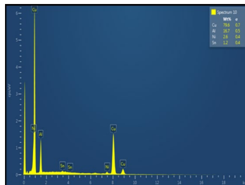
Figure 9 EDS results for S1 alloy.
