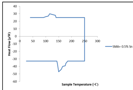
Figure 11: Thermogram of (S1) SMA.
