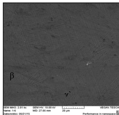
Figure 5: The base (SMA) microstructure
