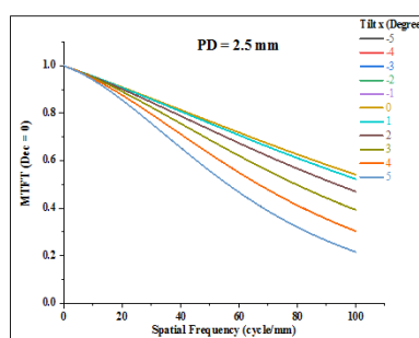
Figure 3: The MTF of eye lens with different tilt (-5 to 5) on X-axis; decenter = 0.0, (a) MTFT, and (b) MTFS
