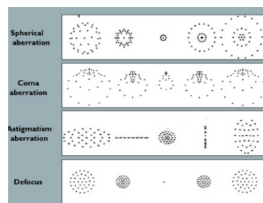
Figure 2: Types of aberration appear in RMS spot size [26]
