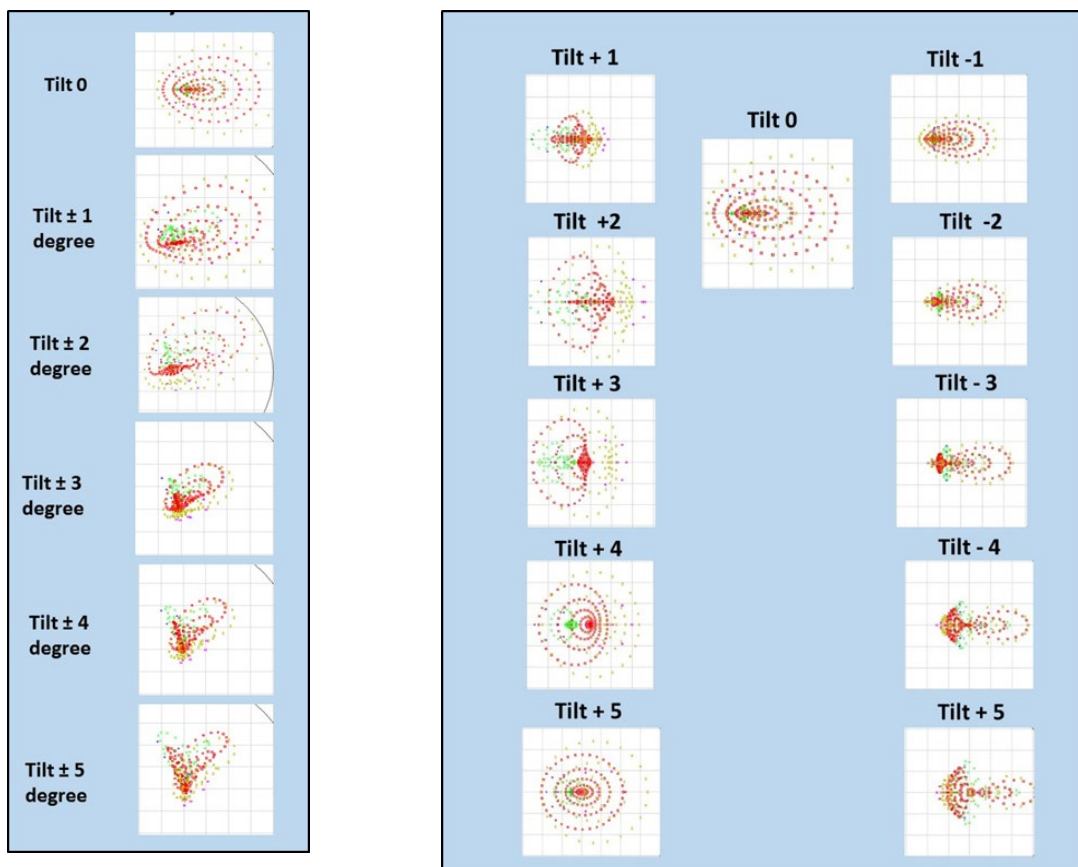
Figure 6: RMS spot size for tilt effect, (a) on X-axis and (b) on Y-axis
