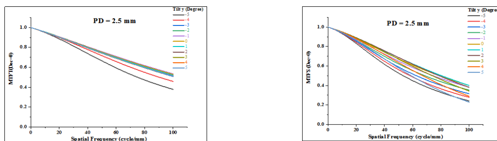
Figure 4: The MTF of eye lens with different tilt (-5 to 5) on Y-axis; decenter =0.0, (a) MTFT, and (b) MTFS
