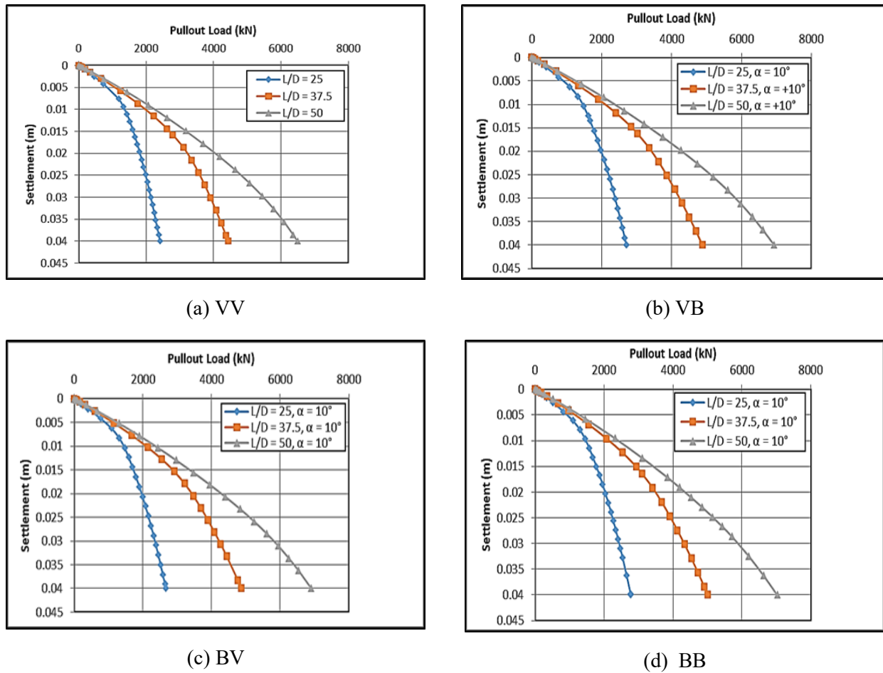
Figure 3: Load-settlement curves for 2 \times 1 pile groups constructed in soil with RD = 80\% at \alpha = 10^\circ : a) VV, b) VB c), BV d), BB
