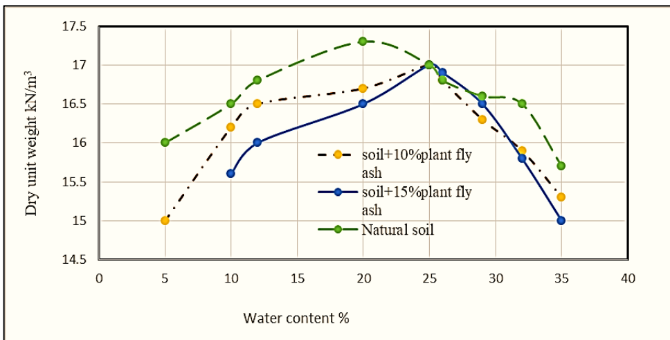
Figure 6: Variation of the dry density with moisture content for different (C/S) and plant fly ash (PFA) presents
