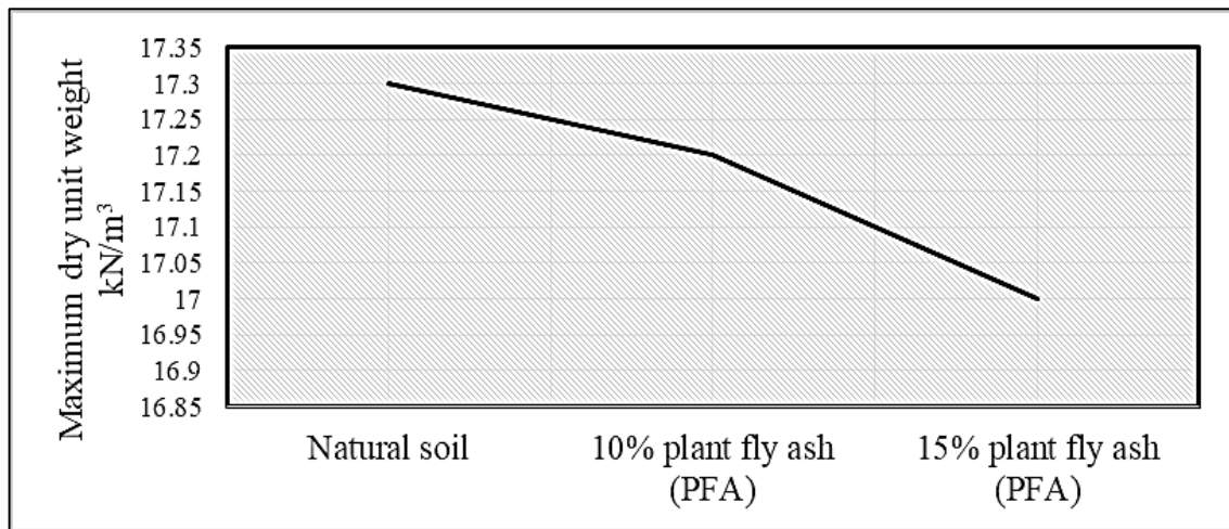
Figure 8: Variation of the maximum dry density for different (C/S) and plant fly ash (PFA) presents
