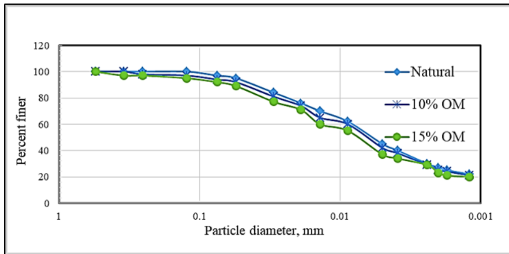
Figure 3: Grain size distribution of the treated and untreated soil
