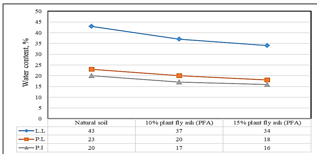
Figure 4: Effect of cement paste and plant fly ash (PFA) content on Atterberg limits
