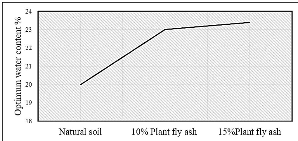
Figure 7: Variation of the optimum water content with different % of additive (C/S) and plant fly ash (PFA) presents
