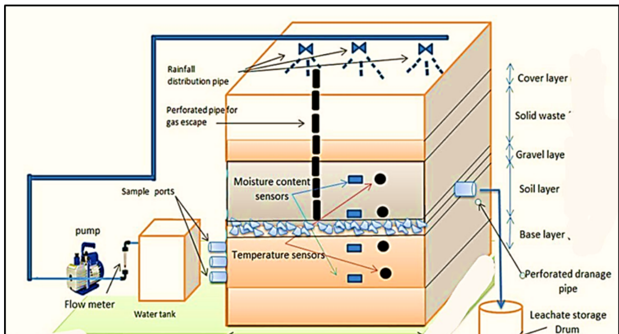
Figure 2: Pilot-scale lysimeter drawing
