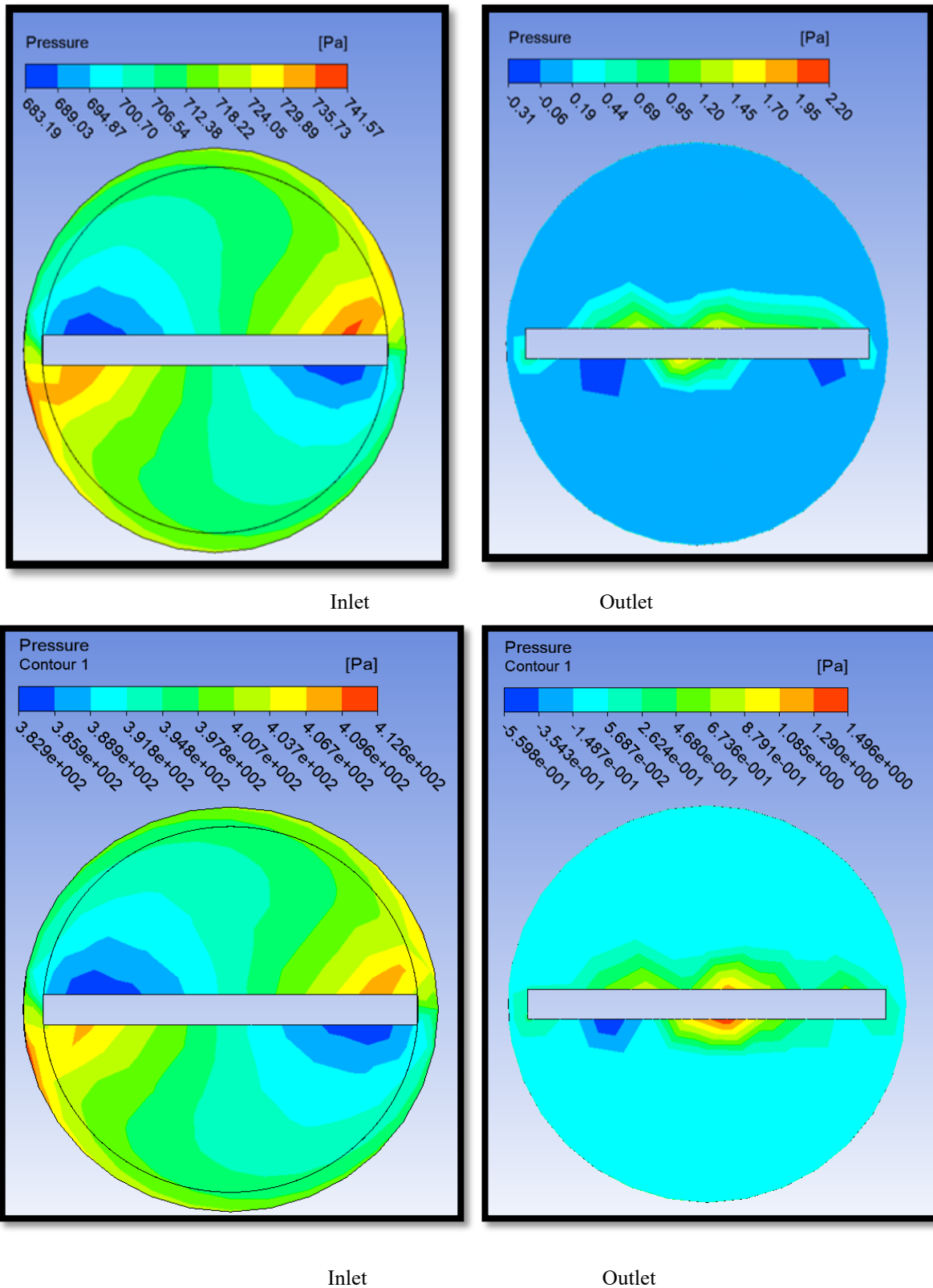
Figure 17: a. Pressure contours for the hybrid nanofluid ( \phi=1.8\% ) and ( Re=8320 ), b. Pressure contours for the distilled water at ( Re=5940 )
