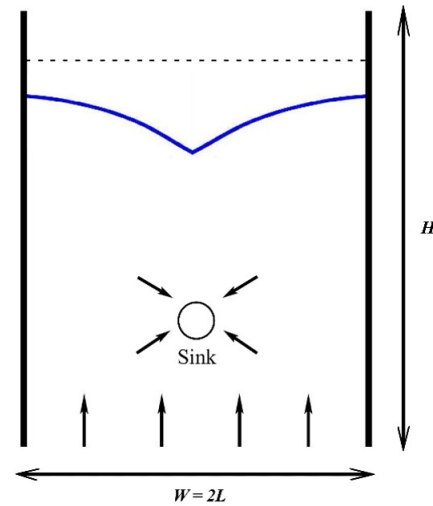
Figure 1. Schematic Representation of the Groundwater Flow Problem Configuration in a Two-dimensional, Vertical Column within a Homogeneous Porous Medium.
