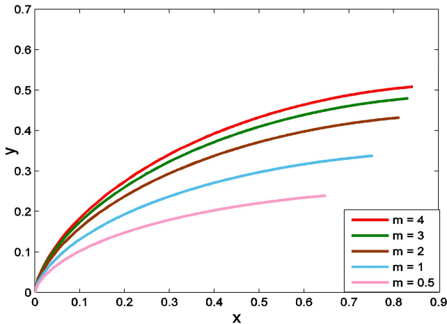
Figure 4. Interface Shape for Hodograph Critical Flow Solution.
