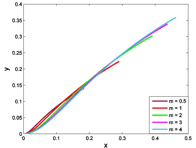
Figure 2. phreatic Surface for Different m Value.
