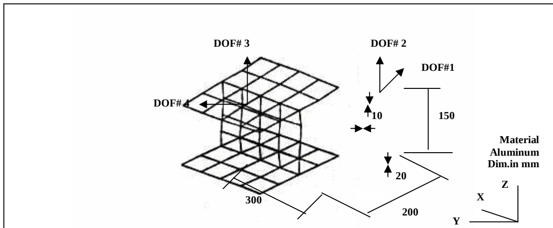
Fig. 22 Test structure
