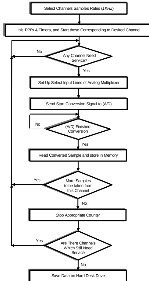
Fig.4 Flow chart of data acquisition software programs.
