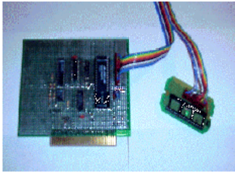
Fig.3 Data acquisition system.
