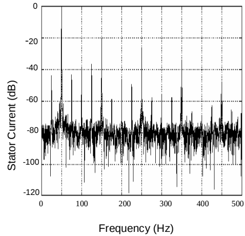
Fig.12 Stator current power spectra in the case of stator voltage unbalance.
