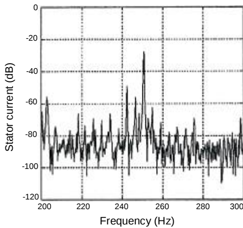
Fig.11 Stator current power spectra for frequencies more than 200Hz.
