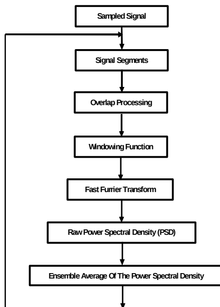
Fig. 5 Steps for estimating the power spectral density (PSD).
