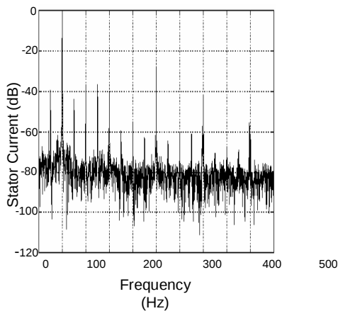
Fig.7 Full-load motor stator current spectra for healthy case.
