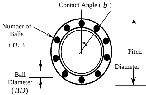
Fig.1 Ball bearing dimensions.
