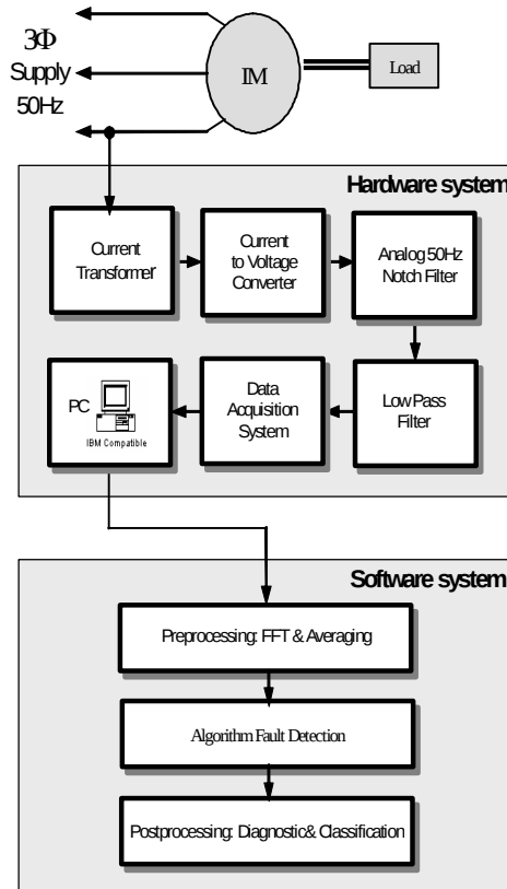
Fig.2 Block diagram of on-line stator current monitoring system.
