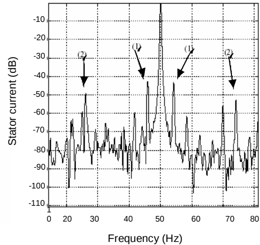
Fig. 10 Stator current power spectra around 50Hz.
