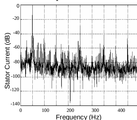
Fig. 13 Stator current power spectra in the case of open phase.
