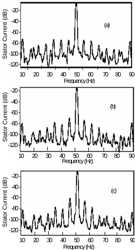
Fig. 9 Stator current power spectra around 50Hz with one,(b)two ,and (c) three adjacent broken bars.
