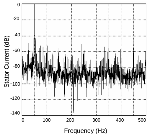
Fig. 8 Full-load motor stator current spectra with one broken rotor bar.
