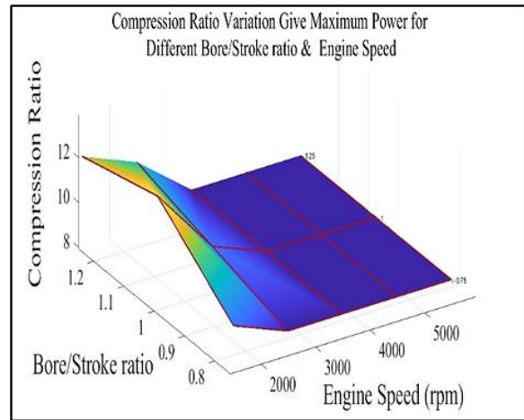
Figure 17: Compression ratio variation gives Maximum for different cylinder bore/stroke ratios for different cylinder bore/stroke ratios
