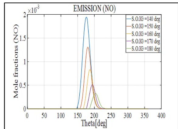
Figure 23: Emissions of NO for different start of ignition
