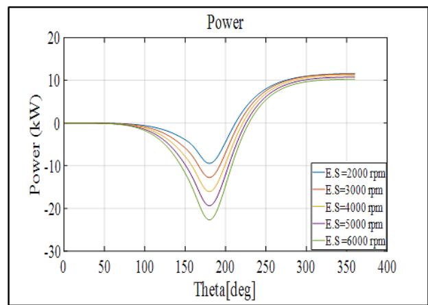
Figure 5: Cumulative engine power for different engine speeds
