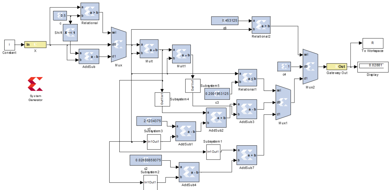
Figure 10: Bell MF based on decomposition and shift-add techniques
