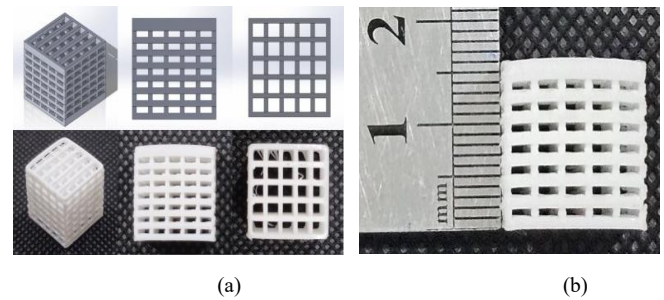
Figure 1. (a) Design of the sample from different views and (b) dimensions of the sample
