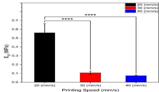
Figure 25. Plateau stiffness of samples printed with printing speeds of (20, 30 and 40 mm/s).
