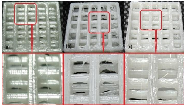
Figure 3. Effect of layer thickness on the structure of the specimens (a) 0.1mm layer thickness, (b) 0.2mm layer thickness, and (c) 0.3mm layer thickness
