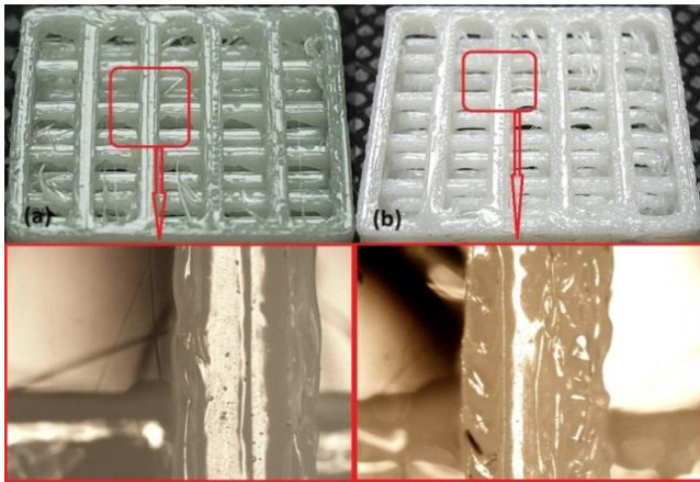
Figure 8. Top view the texture of samples printed with (a) 20 mm/s and (b) 40 mm/s.
