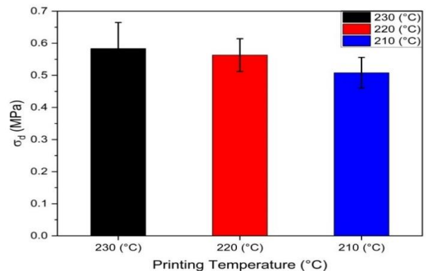
Figure 21. Densification stress of samples printed with printing temperatures of (210, 220 and 230 °C).
