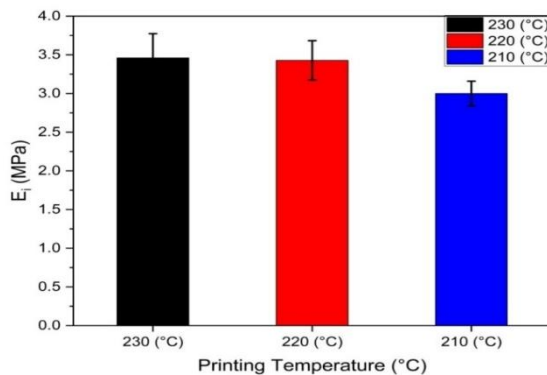
Figure 18. Elastic stiffness of samples printed with printing temperatures of (210, 220 and 230 °C).
