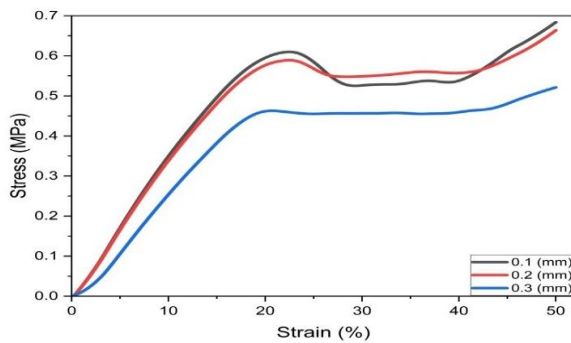
Figure 17. Stress-strain curves of samples printed with layer thicknesses of (0.1, 0.2 and 0.3 mm).
