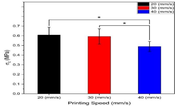
Figure 24. Collapse stress of samples printed with printing speeds of (20, 30 and 40 mm/s).
