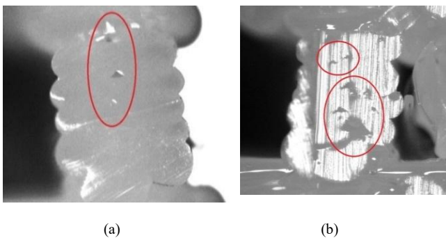
Figure 9. Cross-sectional view of specimens printed with (a) 20 mm/s and (b) 40 mm/s
