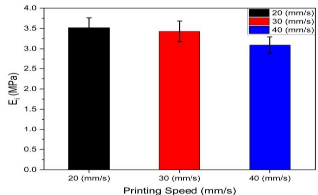
Figure 26. Densification stress of samples printed with printing speeds of (20, 30 and 40 mm/s).
