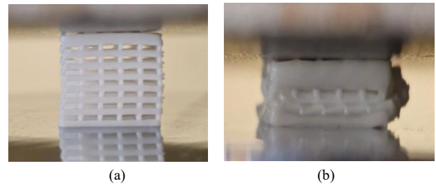
Figure 10. (a) specimen before compression and (b) specimen after
