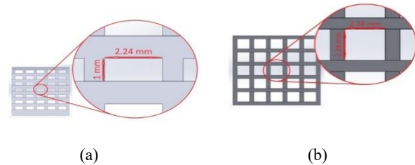
Figure 2. (a) Dimensions of the pores at the sides of the sample and (b) Dimensions of the pores at the top and bottom of sample.
