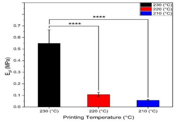
Figure 20. Plateau stiffness of samples printed with printing temperatures of (210, 220 and 230 °C).
