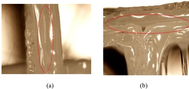
Figure 4. Effect of 0.3 mm layer thickness on the structure (a) strut area and (b) join area.
