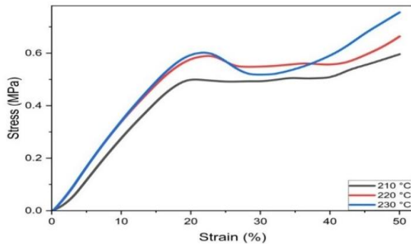
Figure 22. Stress-strain curves of samples printed with printing temperatures of (210, 220 and 230 °C).
