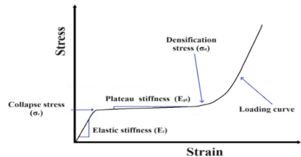
Figure 11. Stress-strain curve for the elastic material in compression with definition of material characteristics.
