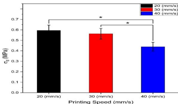
Figure 23. Elastic stiffness of samples printed with printing speeds of (20, 30 and 40 mm/s).
