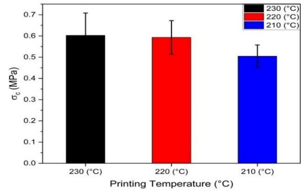
Figure 19. Collapse stress of samples printed with printing temperatures of (210, 220 and 230 °C).
