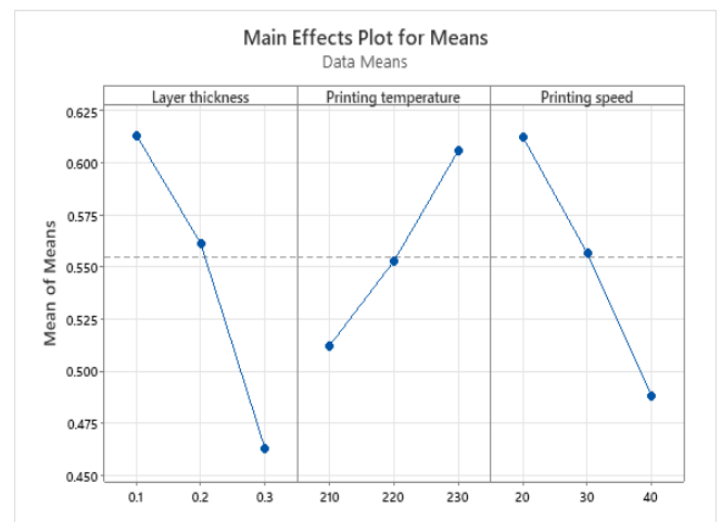
Figure 29. DOE Main effect plot for collapse stress
