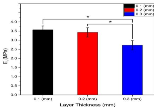
Figure 13. Elastic stiffness of samples printed with layer thicknesses of (0.1, 0.2 and 0.3 mm). Note: An asterisk indicates the digits of statistically significant difference (*= p < 0.05 , **= p < 0.01 , ***= p < 0.001 , and ****= p < 0.0001 )
