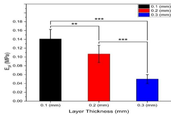
Figure 14. Collapse stress of samples printed with layer thickness (0.1, 0.2 and 0.3 mm).
