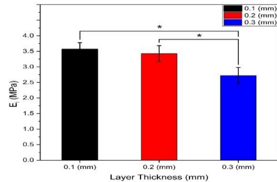
Figure 15. Plateau stiffness of samples printed with layer thicknesses of (0.1, 0.2 and 0.3 mm).
