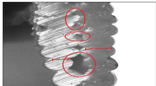
Figure 7. Cross-sectional view of the specimen printed with 210 °C.
