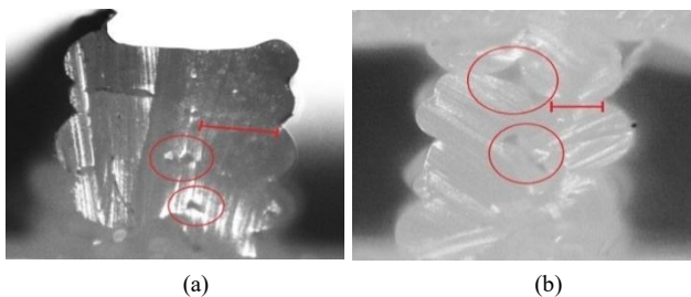
Figure 5. Cross-sectional view of contact area and porosities in (a) 0.2mm and (b) 0.3mm specimens
