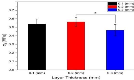
Figure 16. Densification stress of samples printed with layer thicknesses of (0.1, 0.2 and 0.3 mm).
