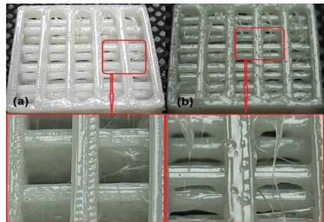
Figure 6. Illustration the top view texture of the printed specimens with (a) 210 °C and (b) 230 °C.
