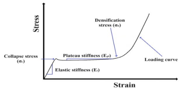
Figure 12. Stress-strain curve for the elastic-plastic material in compression with definition of material characteristics.
