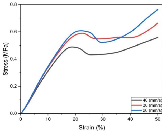
Figure 27. Stress-strain curves of samples printed with printing speeds of (20, 30 and 40 mm/s).
