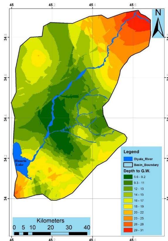
Fig. 3. Spatial distribution of depths to groundwater in the studied area.
