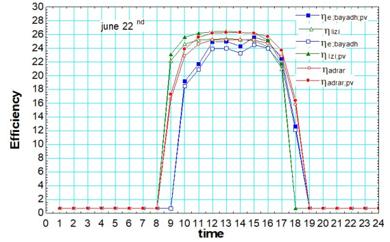
Figure 8. Daily performance trend of the plant on June 22 in Adrar, Illizi, and El Bayadh.
