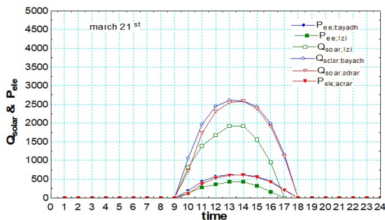
Figure 11. Variation of electric power and solar power on March 21 in: Adrar, Illizi, and El Bayadh.
