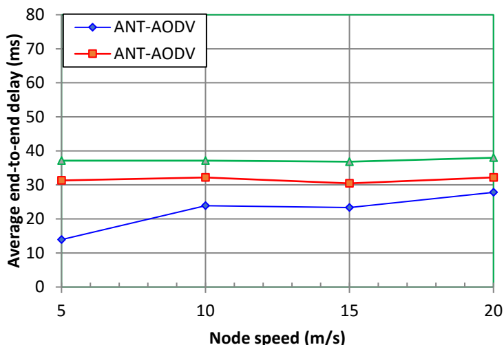
Figure 3. Average End-to-End Delay
