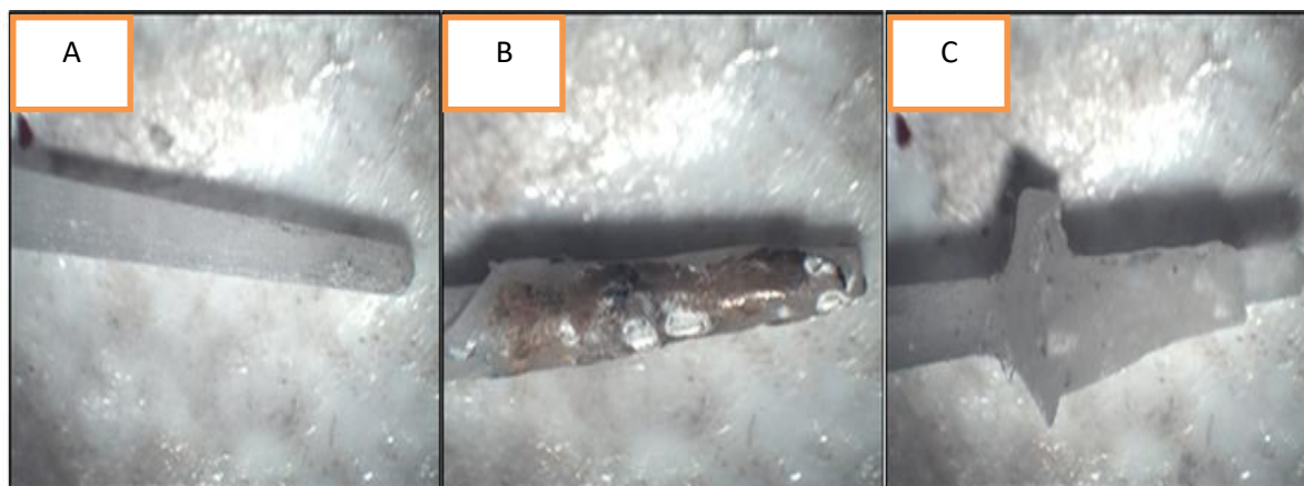
Figure (5): mode of failure under stereomicroscope: (A) Adhesive, (B) cohesive, (C) mixed type.
