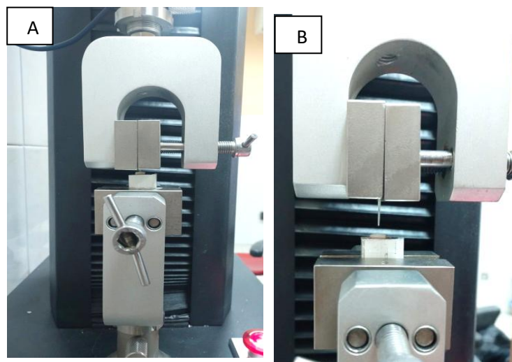
Figure (3): Universal testing machine with specimen. Engagement of fiber post in machine (A), dislodgement of fiber post (B).
