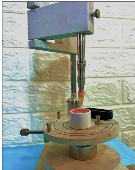
Figure (1): Placement of specimen inside acrylic mold with aid of dental surveyor
