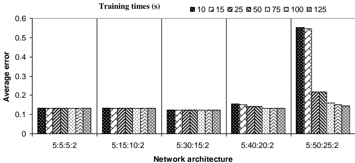
Figure 5. Average error for the best architecture for each length of training time for the prediction network for the permeate flux and salt passage trained with two-hidden-layer configurations.
