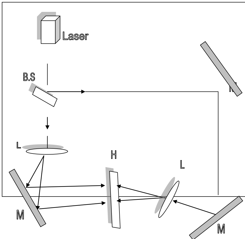
Figure(1)recording Reflection grating fabrication
