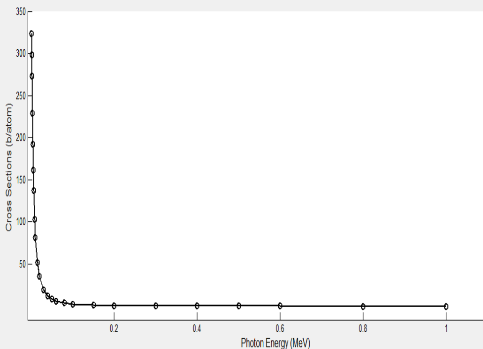
Fig.(2):show the coherent differential cross section versus the photon energies for Vanadium ^{51}\text{V}_{23} .
