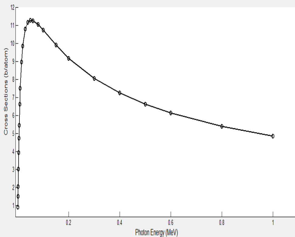
Fig.(3):show the Incoherent differential cross section versus the photon energies for Vanadium ^{51}\text{V}_{23} .
