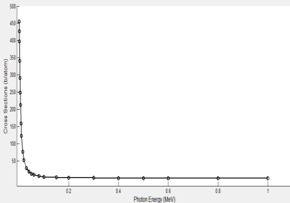
Fig.(4):show the coherent differential cross section versus the photon energies for Cobalt ^{59}\text{Co}_{27} .
