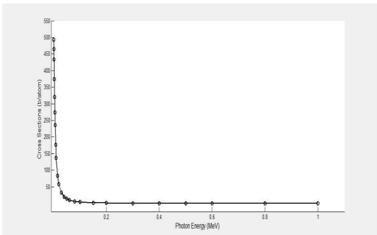
Fig.(6):show the coherent differential cross section versus the photon energies for Nickel ^{59}\text{Ni}_{28} .
