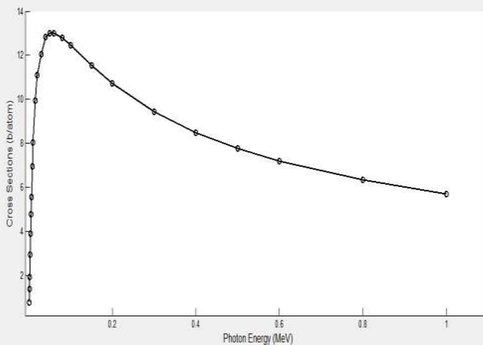
Fig.(5):show the Incoherent differential cross section versus the photon energies for Cobalt ^{59}\text{Co}_{27} .
