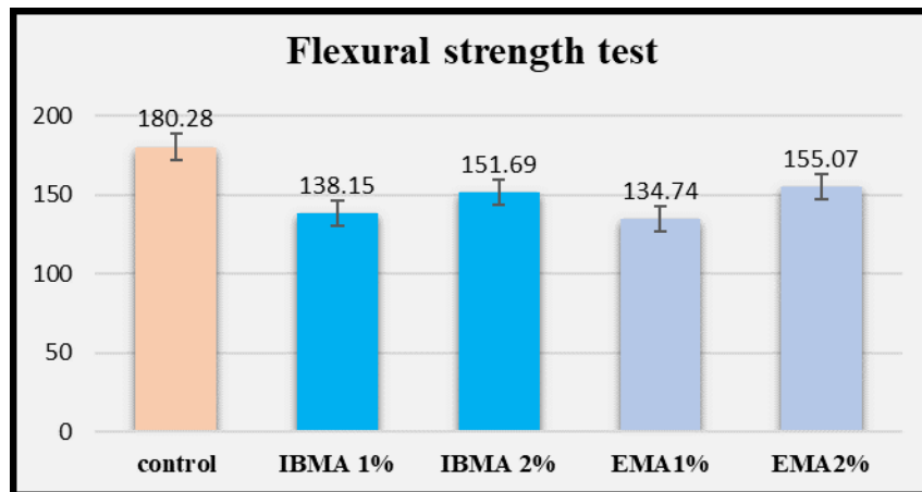
Figure (3): Bar chart representing mean values of Transverse strength test for the studied group
