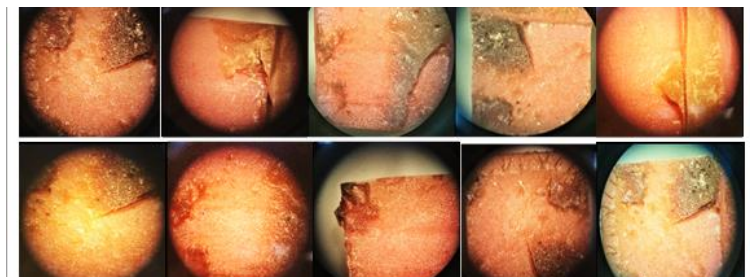
Fig. (10): Mode of failure of specimens shear bond strength (Neem 10 % wt.)
