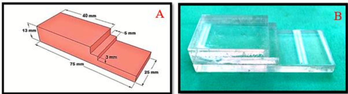
Fig. (3): (A) Dimensions of specimen shear bond strength, (B) Plastic pattern of specimen shear bond strength
