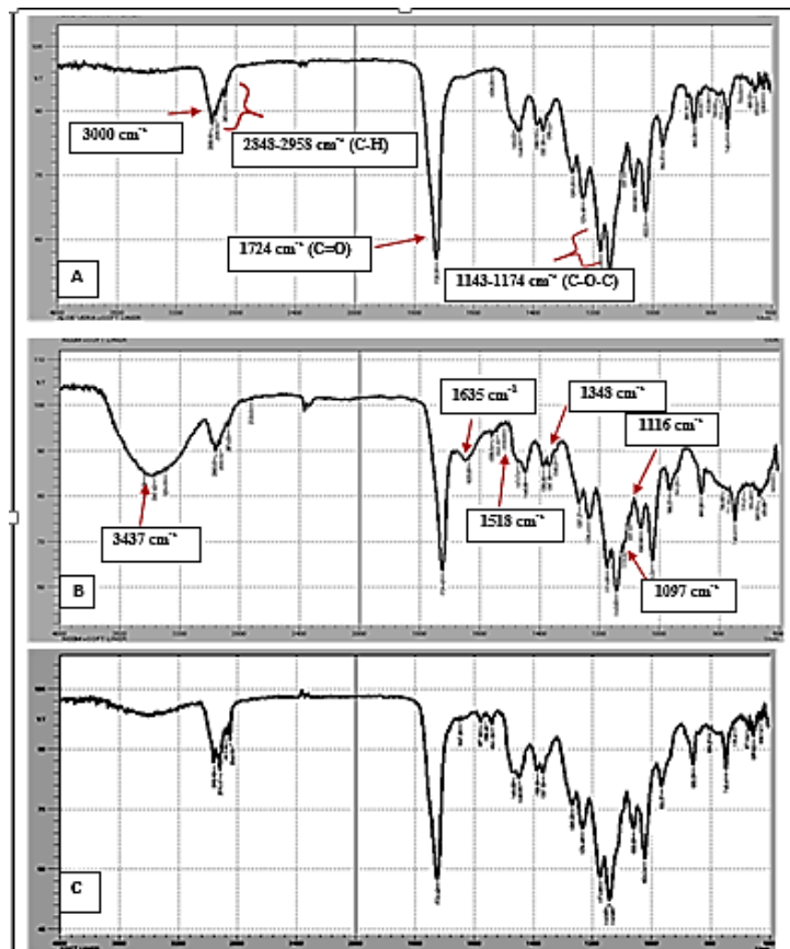
Fig. (12): FTIR analyzer (A) soft liner specimen (control) (B) specimen after incorporation of 10% of Neem (C) specimen after incorporation of 10% of Aloe
