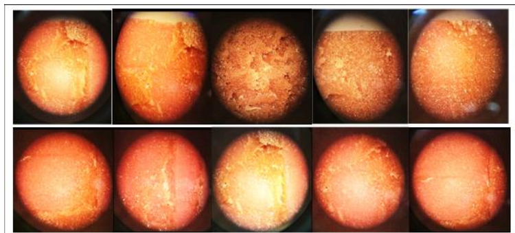
Fig. (11): Mode of failure of specimens shear bond strength (Aloe vera 10 % wt.)
