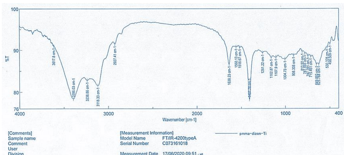
Fig. (3): FTIR spectrum of titanium alloy.
