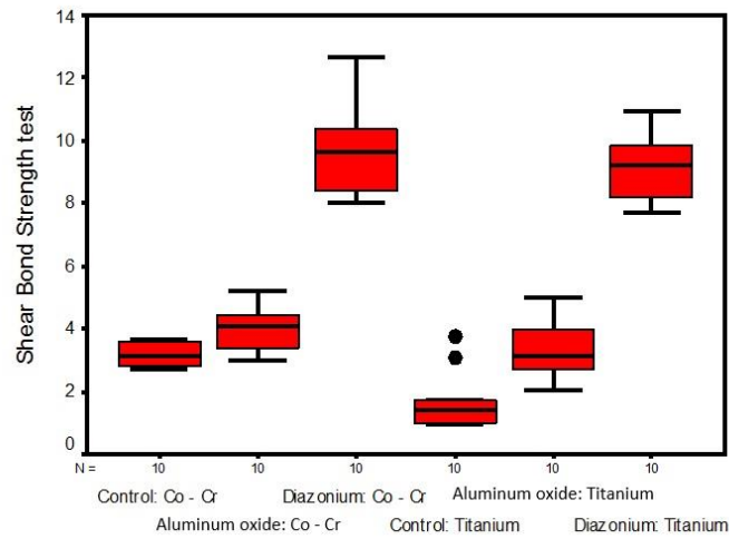
Fig. (1): Box plot for shear bond strength test.
