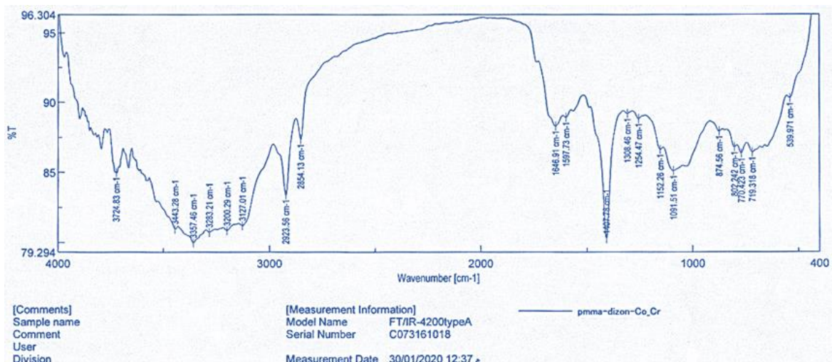
Fig. (2): FTIR spectrum of Co/Cr alloy.
