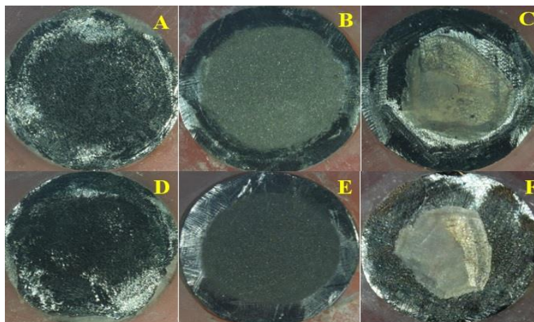
Fig. (2): The mode of failure image.
