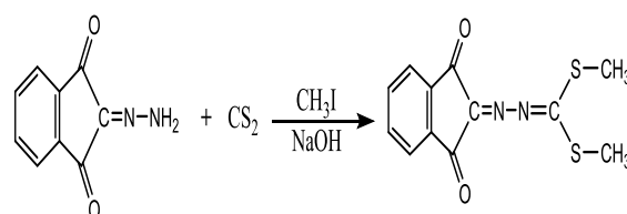
dimethyl (1,3-dioxo-1,3-dihydro-2H-inden-2-ylidene)carbonohydrazonodithioate
