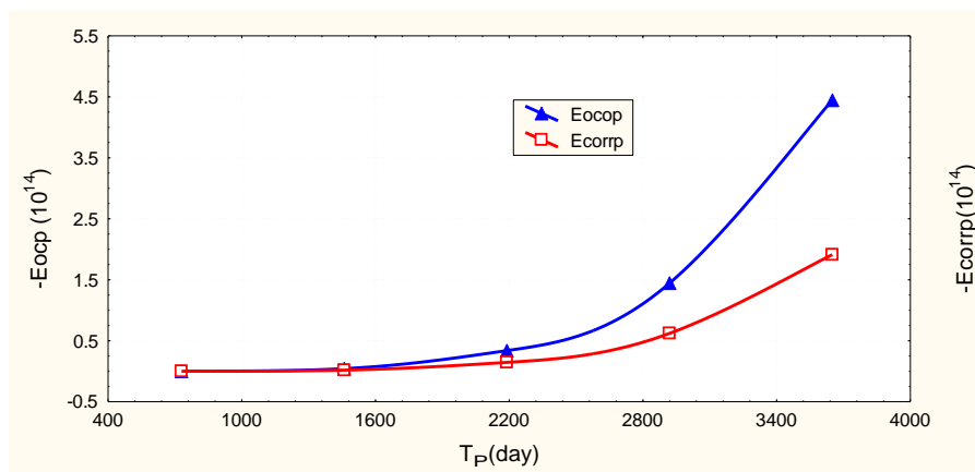
Fig. (4):- Predicted values of E_{oc} and E_{corr} for amalgam in artificial saliva at long time after filling.
