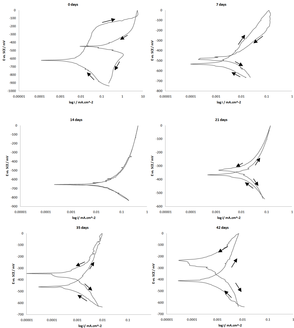
Fig. (3):- Cyclic polarization for amalgam in artificial saliva at different time after filling.
