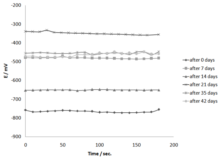
Fig.(1):- The variation of open circuit potential – time for amalgam in artificial saliva.
