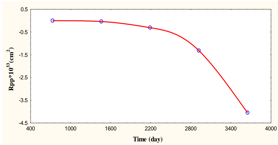
Fig. (5):- Predicted values of R_p for amalgam in artificial saliva at long time after filling.
