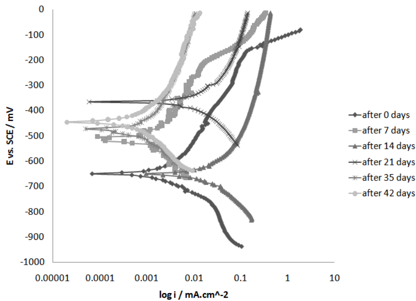
Fig. (2):- Potentiodynamic polarization for amalgam in artificial saliva at different time after filling.
