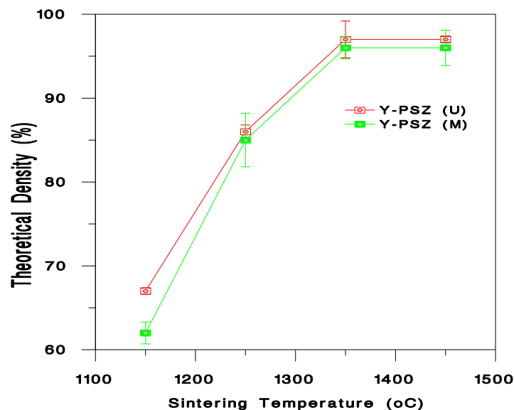
Fig. (1):- The effect of sintering temperature on the % theoretical density of ZrO 2 -U and ZrO 2 -M samples, fired for 6 hrs in an air atmosphere (Y-PSZ is yttrium partially stabilised zirconia).
