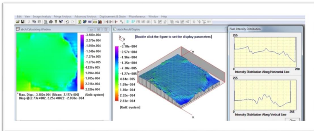
Fig.(3):- MOIRE Software Package system.
