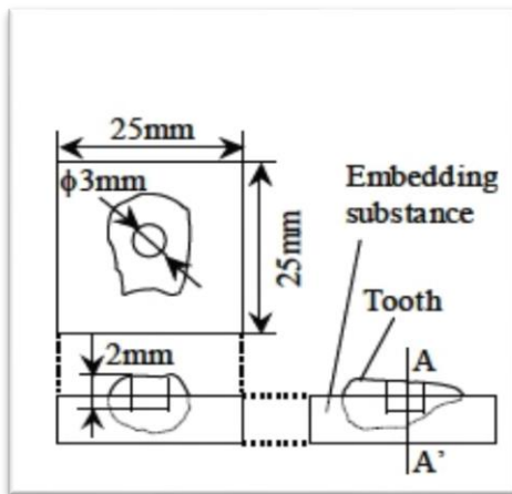
Fig. (1):- Specimen geometries.
