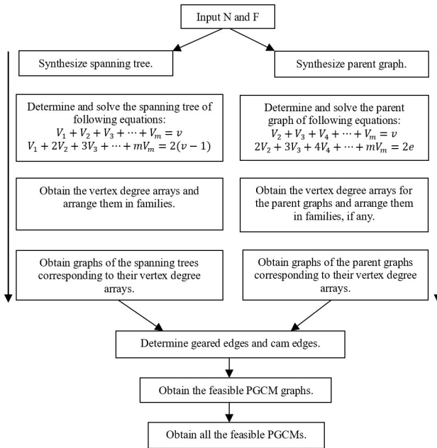
Figure 16. Flow chart for the structure synthesis of PGCMs.
