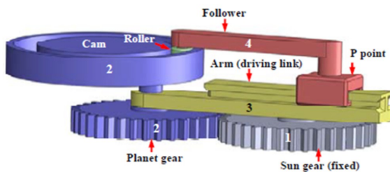
Figure 12. Exact path generation mechanism [17].
