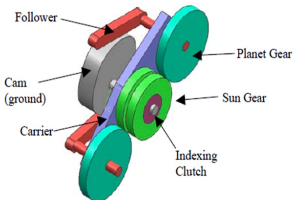
Figure 5. Simplified depiction of the IVT [5].
