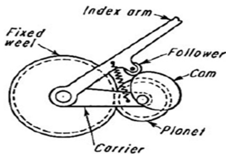
Figure 11. Planetary Gear-Cam mechanism with fixed sun gear.
