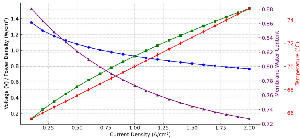
Figure 1. Correlation between voltage, power density, membrane water content, and temperature distribution of a PEMFC under simulated marine operating conditions.
