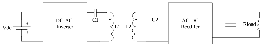
Figure 4. Block schematic of the proposed system.
