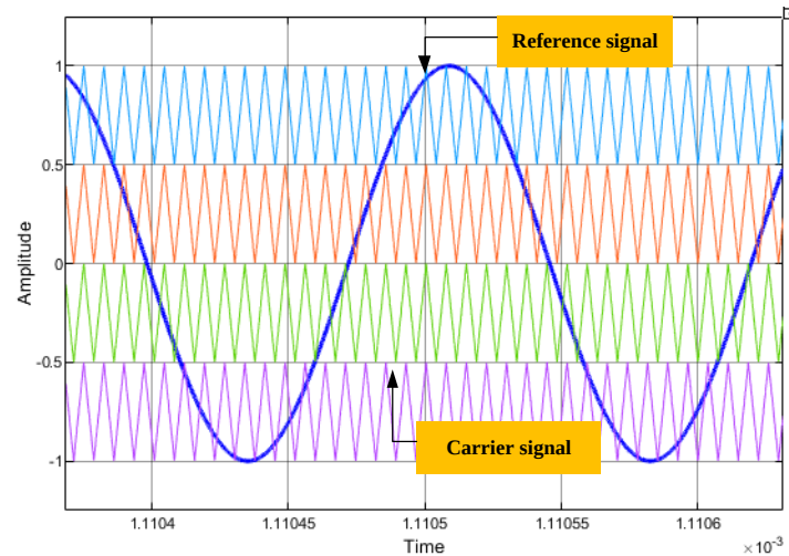
Figure 6. PD modulation technique.
