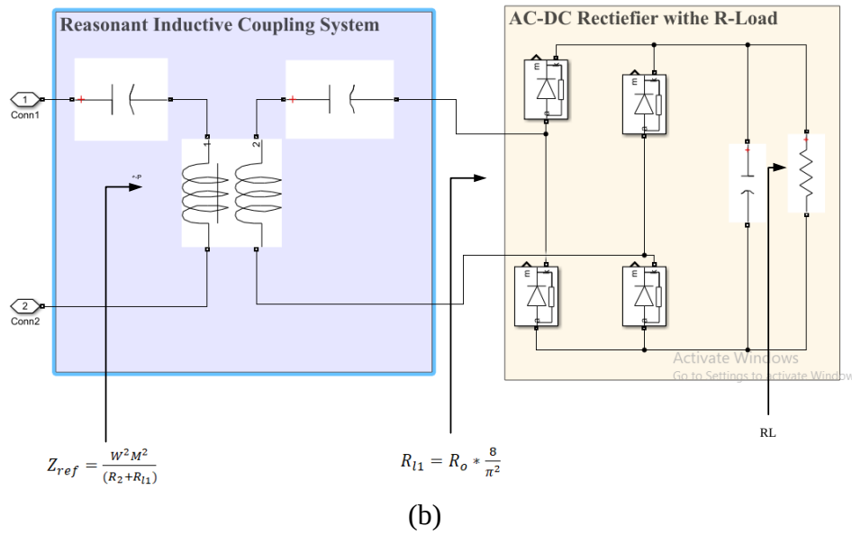
Figure10. a) Simulink model of the proposed system with a class E inverter
