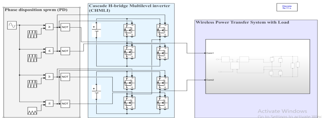
Figure 7. Model of the proposed system with CHMLI in Simulink.
