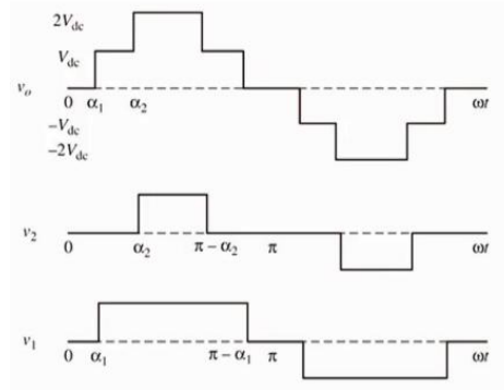
Figure 8. Output voltage of CHMLI.
