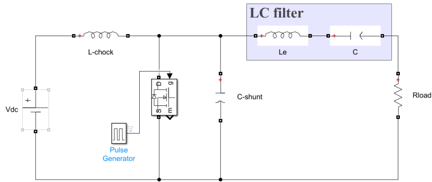
Figure 9. Circuit topology of class E inverter.
