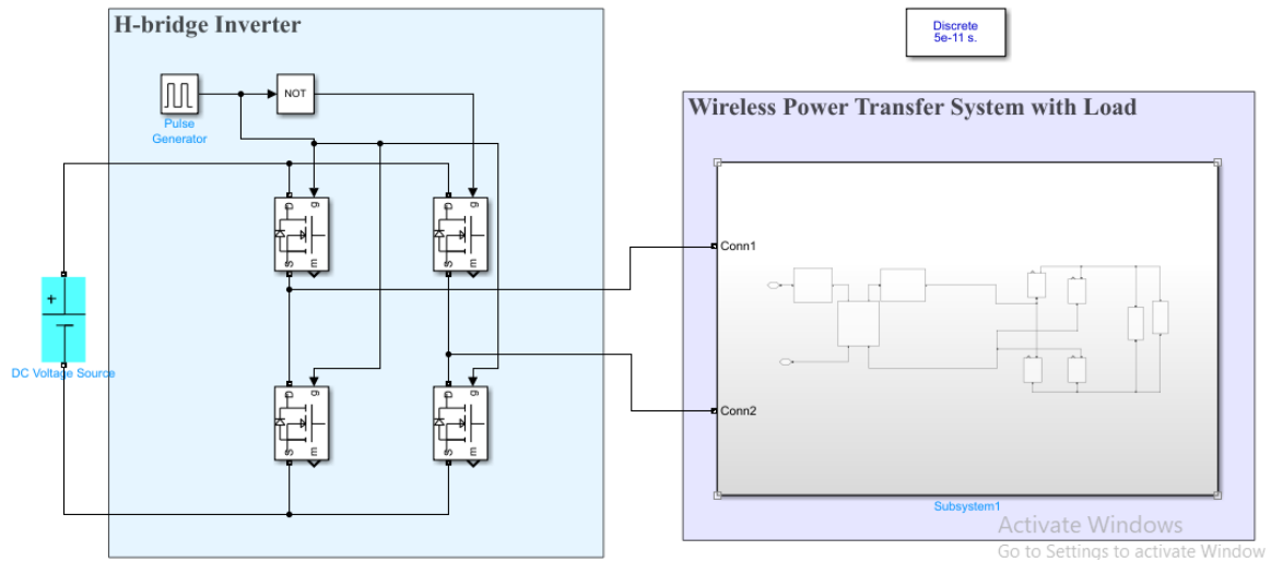
Figure 5. Model of the proposed system with an H-bridge inverter in Simulink.
