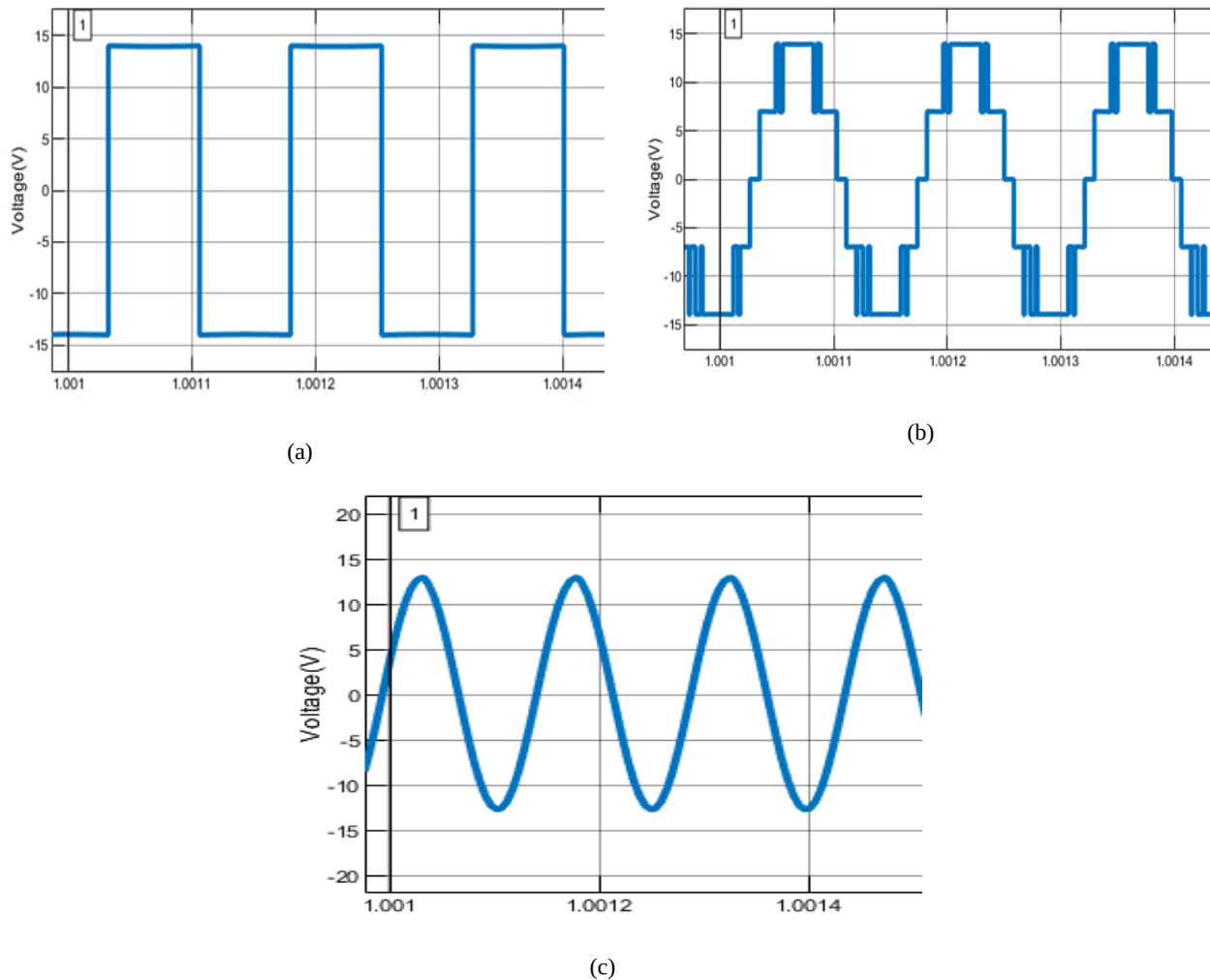
Figure 11. output voltage for three inverter topologies, (a) H-bridge inverter, (b) five-level inverter, (c) class-E inverter.
