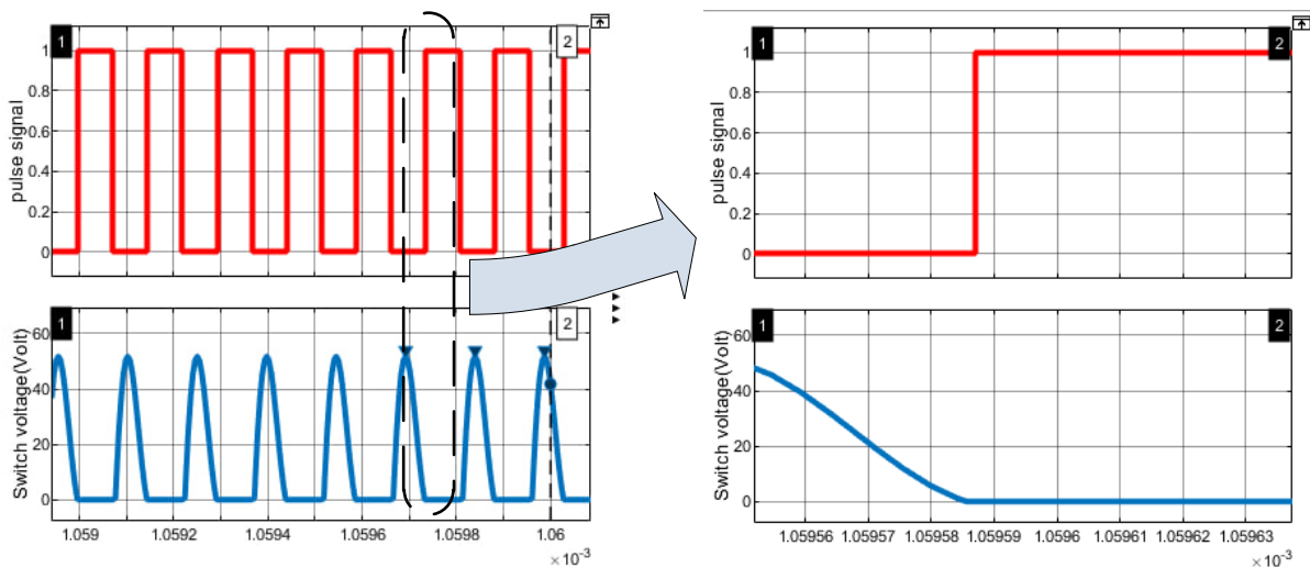
Figure12. Achieving of ZVS condition.
