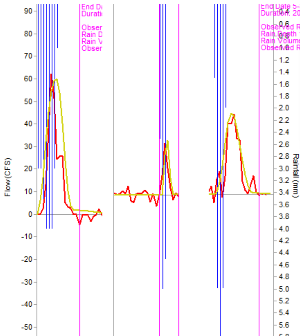
Figure 10. RDII hydrographs calibration in SSOAP.
