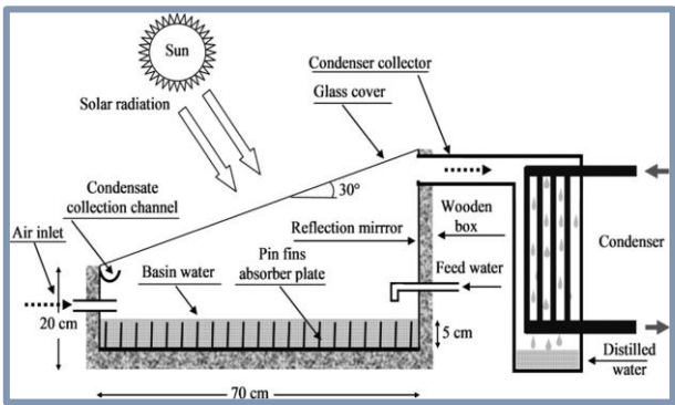
Figure 10. Schematic of solar still with pin fins absorber and external condenser.
