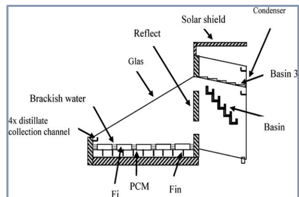
Figure 6. Diagrammatic representation of a solar still with condenser.
