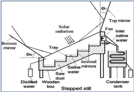
Figure 8. Schematic diagram of stepped solar still with mirrors and condenser.
