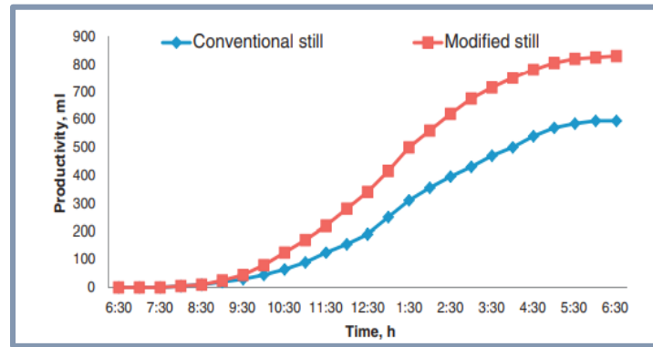
Figure 11. Comparison of modified stills.
