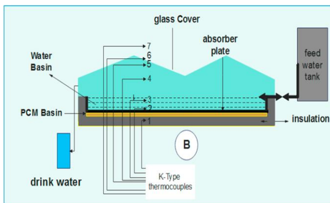
Figure 5. Diagram of a solar still with a condenser and phase change material (PCM).
