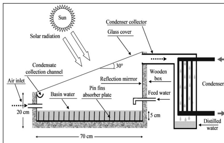
Figure 2. Schematic showing solar still with condenser.
