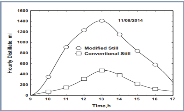
Figure 9. Comparative analysis of simple solar still and modified solar still with condenser.
