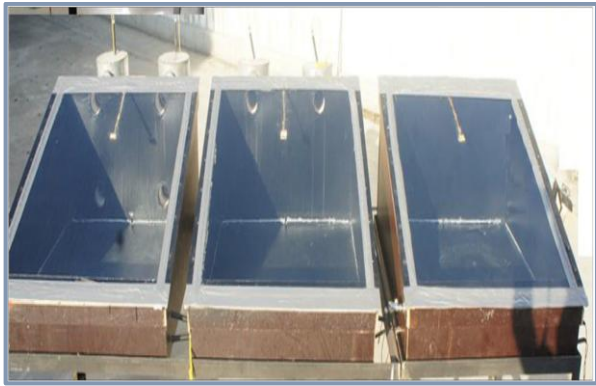
Figure 7. solar still with a novel condenser.
