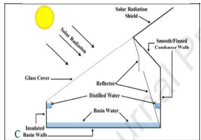
Figure 4. Heat sink condenser solar still
