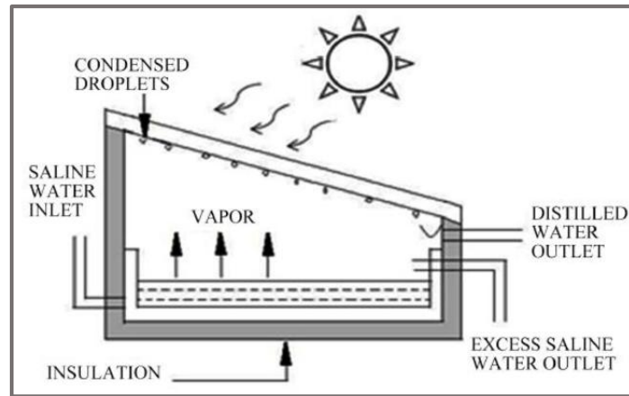
Figure 1. Diagram of a solar still with a single basin.
