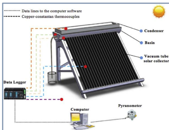
Figure 3. Diagrammatic representation of the solar still connected to the condenser and evacuated tubes.
