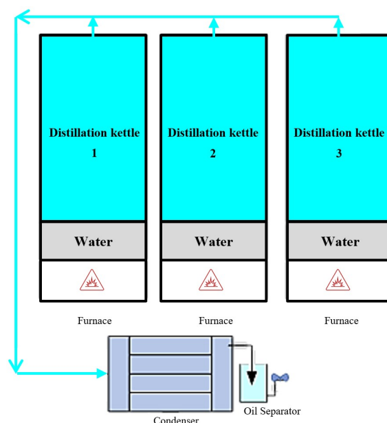
Figure 2. Production process of citronella oil for method 1 (one boiler for one kettle).
