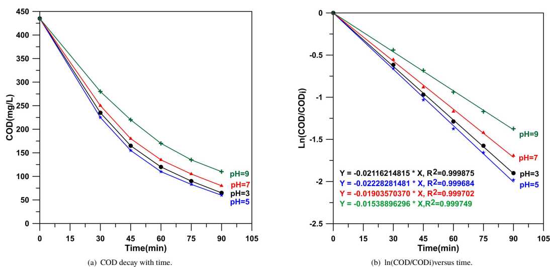
Figure 12. kinetic results for effect of pH.
