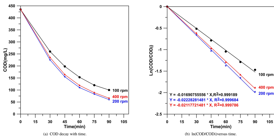
Figure 13. kinetic results for effect of rotation speed.
