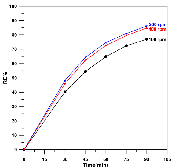
Figure 8. Impact of rotation speed on RE%. 6 \text{ mA/cm}^2 , \text{pH}=5
