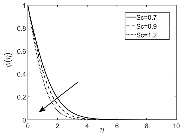
Figure 20. Variations of Concentration with the change in Schmidt number.
