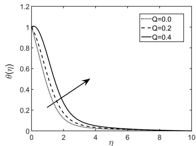
Figure 17. Variations of Temperature with the change in heat source parameter.
