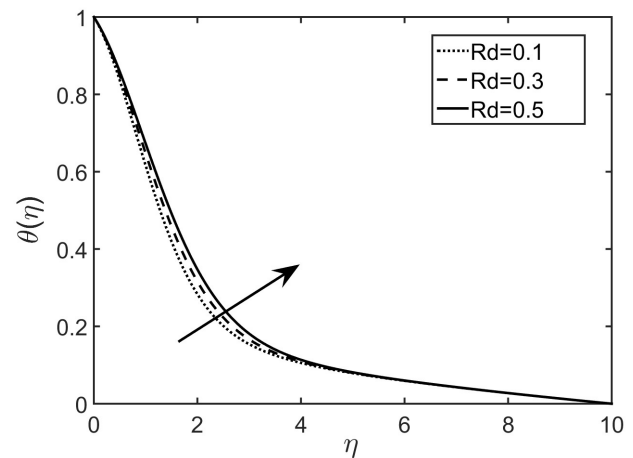
Figure 19. Variations of Temperature with the change in Radiation parameter.
