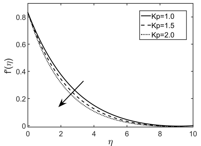
Figure 8. Variations of Velocity with the change in Porous parameter.
