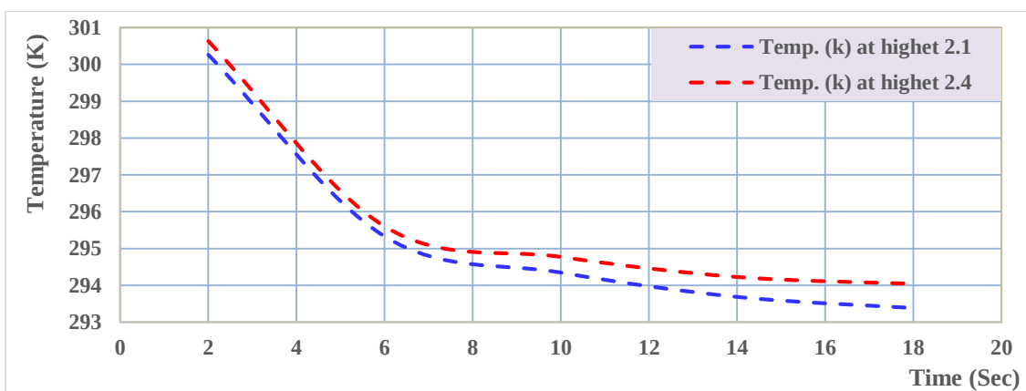
Figure 34. Comparison of all cases (temperature in point (3) in the velocity (6.5 m/s)).
