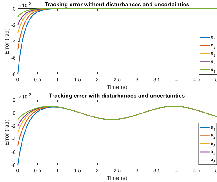
Figure 3. Tracking error with and without disturbance and uncertainty.
